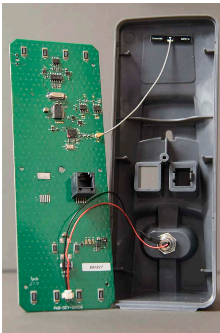
Inside Splayed
