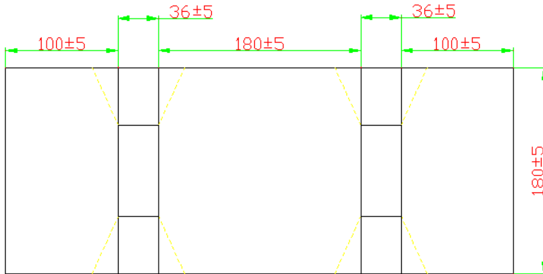
a. Drawing of small size carton in developed view
