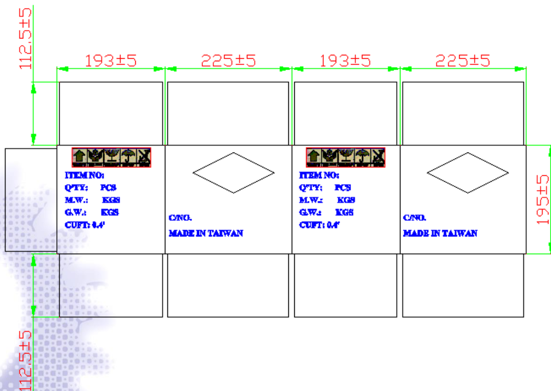
b. Drawing of middle size carton in developed view
