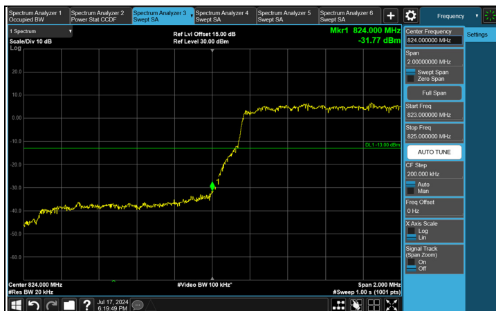
FULL CH 20407 (824.7 MHz)
