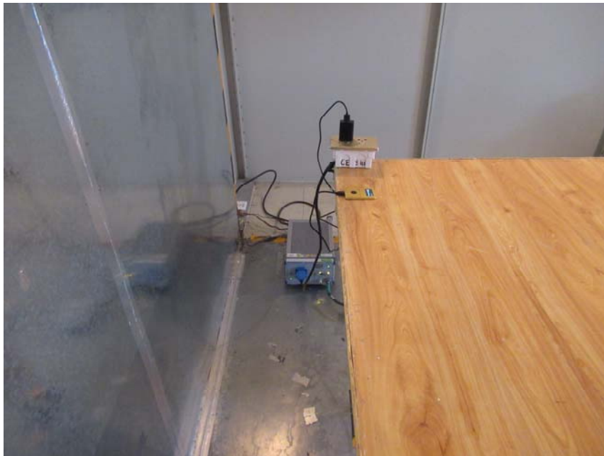
Conducted Emissions -Left Side
