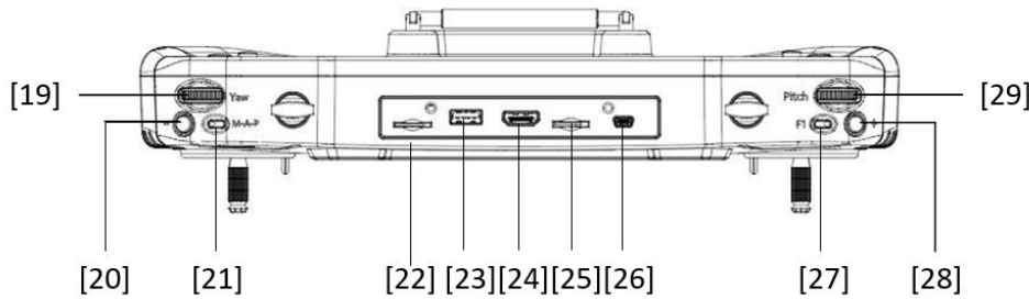
Figure 4 Top Schematic diagram of the Etlas Mobile
