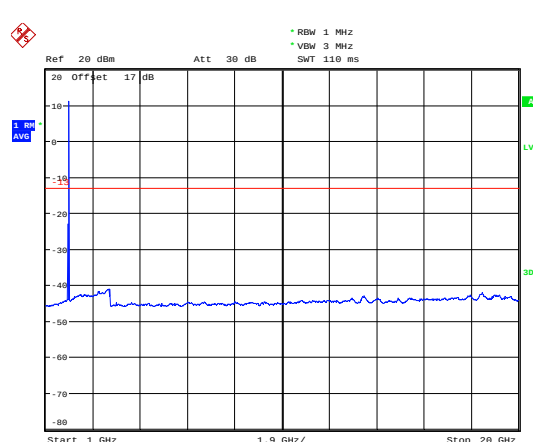
LTE Band 25 1.4MHz CH-High 1GHz~20GHz
