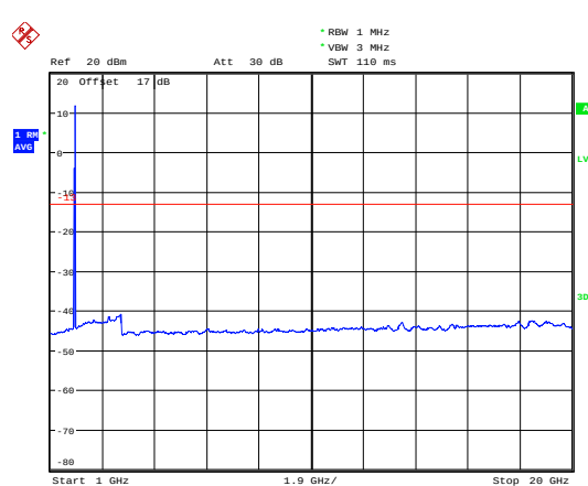
LTE Band 25 1.4MHz CH-Middle 1GHz~20GHz
