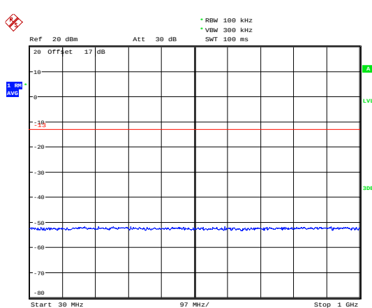
LTE Band 25 1.4MHz CH-Middle 30MHz~1GHz
