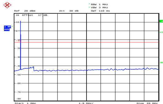
LTE Band 25 1.4MHz CH-Low 1GHz~20GHz
