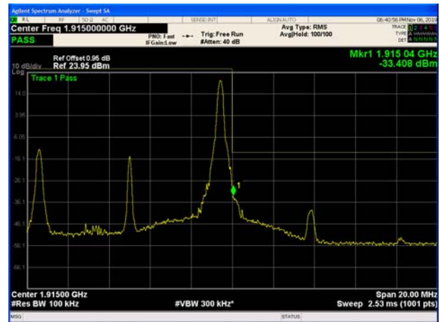
LTE Band 25 10MHz 16QAM 100%RB CH-High
