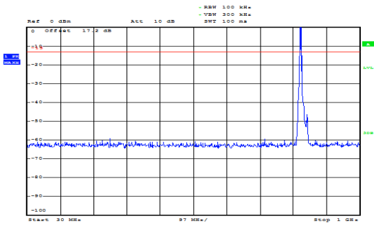
WCDMA Band V CH-Low 30MHz ~ 1GHz
