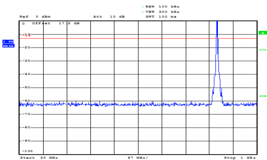
WCDMA Band V CH-Middle 30MHz ~ 1GHz
