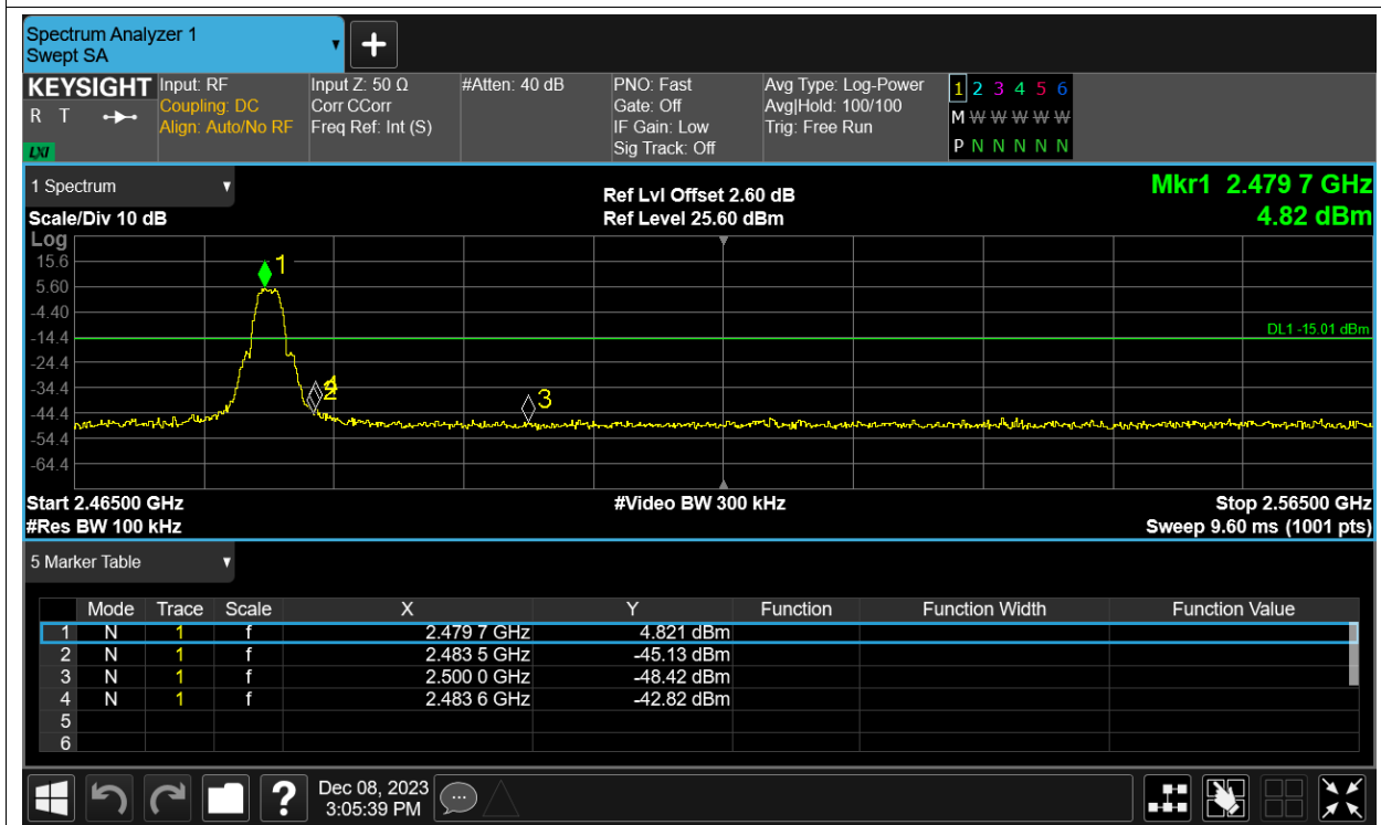
Band Edge NVNT ZigBEE 2480MHz Ant1 Emission
