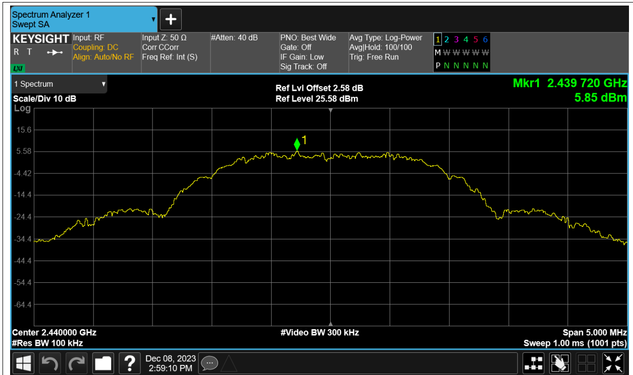
Tx. Spurious NVNT ZigBEE 2440MHz Ant1 Emission
