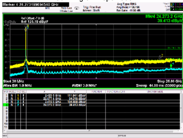
802.11g Ch 2 Spurious
