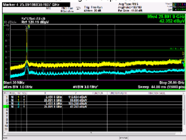
802.11g Ch 10 Spurious
