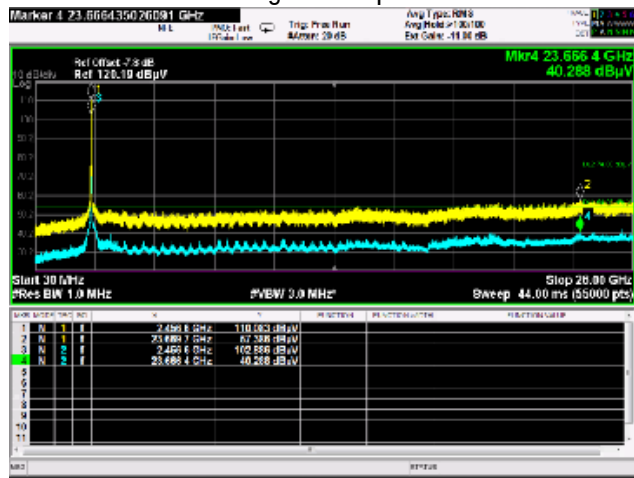
802.11g Ch 11 Spurious
