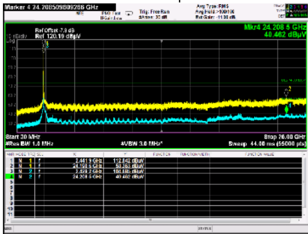
802.11n Ch 6 Spurious
