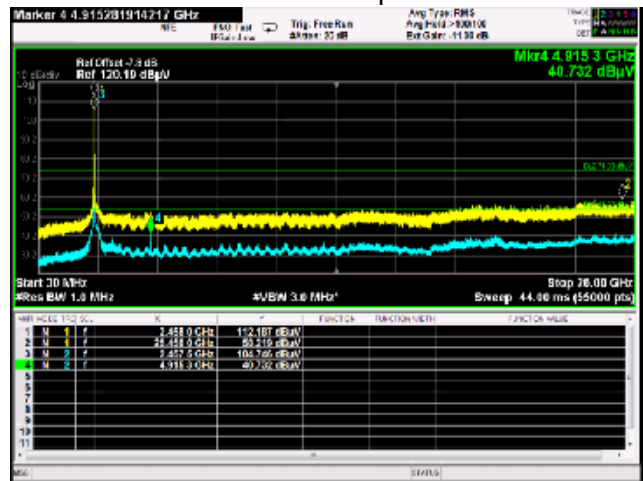
802.11n Ch 10 Spurious
