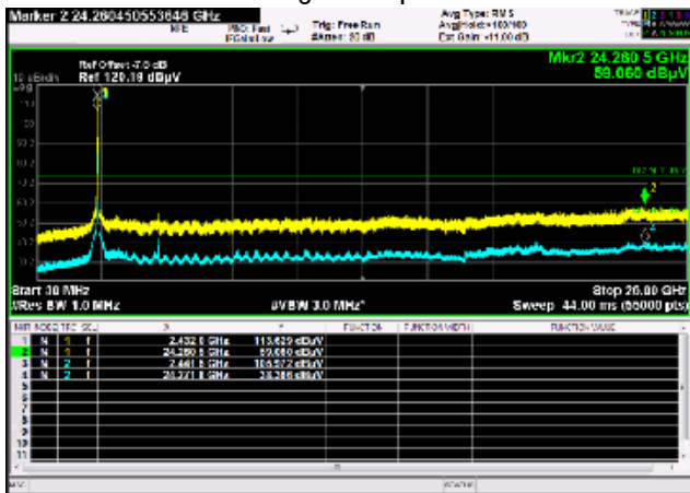
802.11g Ch 6 Spurious
