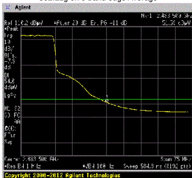
802.11g Ch 9 Band edge Average
