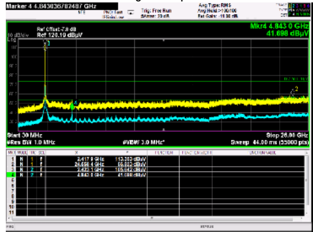
802.11g Ch 3 Spurious
