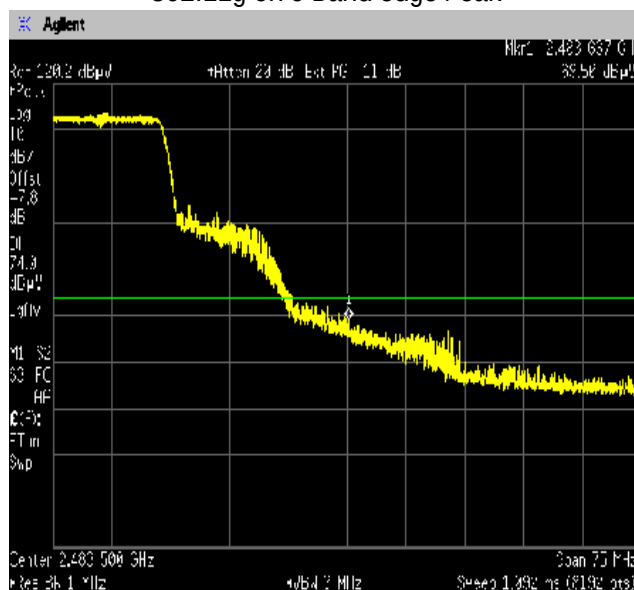
802.11g Ch 9 Band edge Peak
