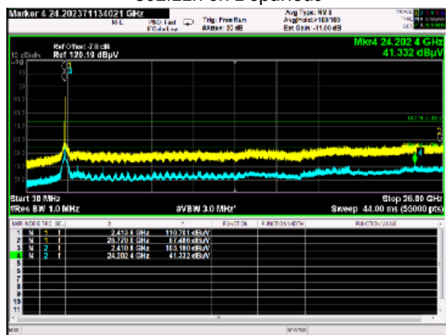
802.11n Ch 1 Spurious
