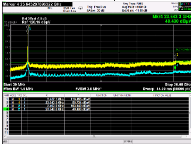
802.11n Ch 11 Spurious
