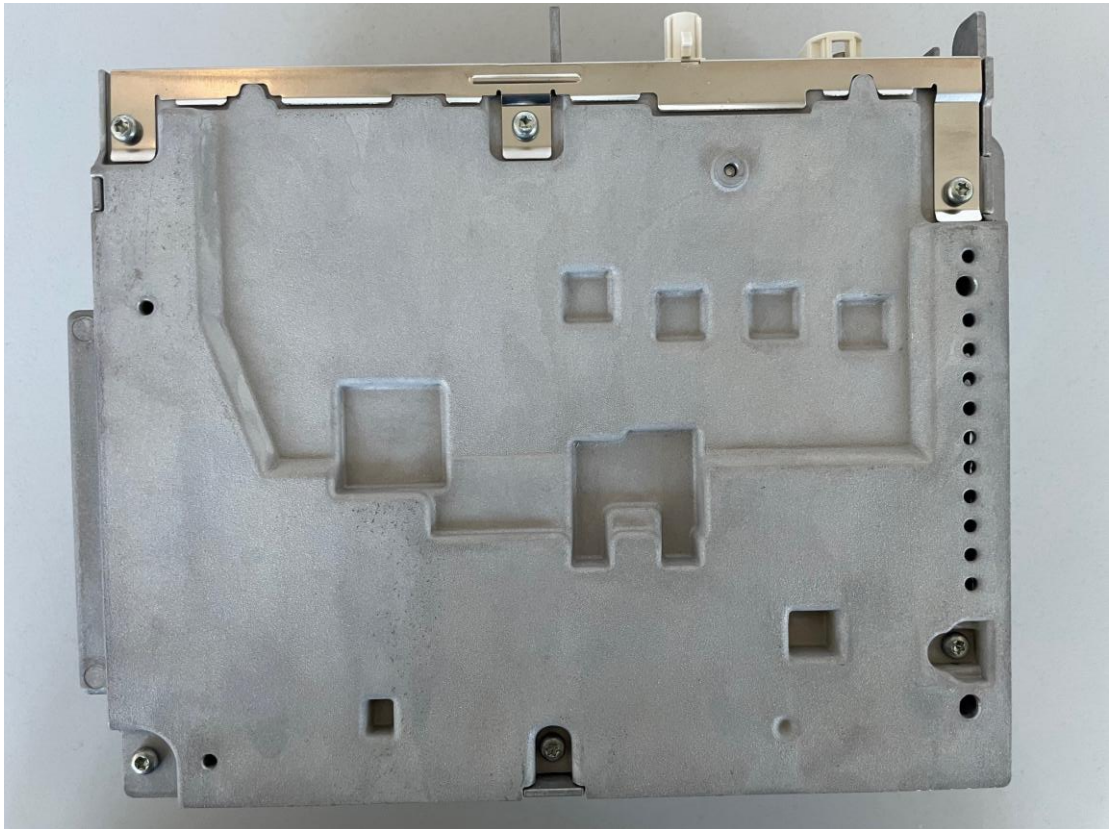
Buttom
