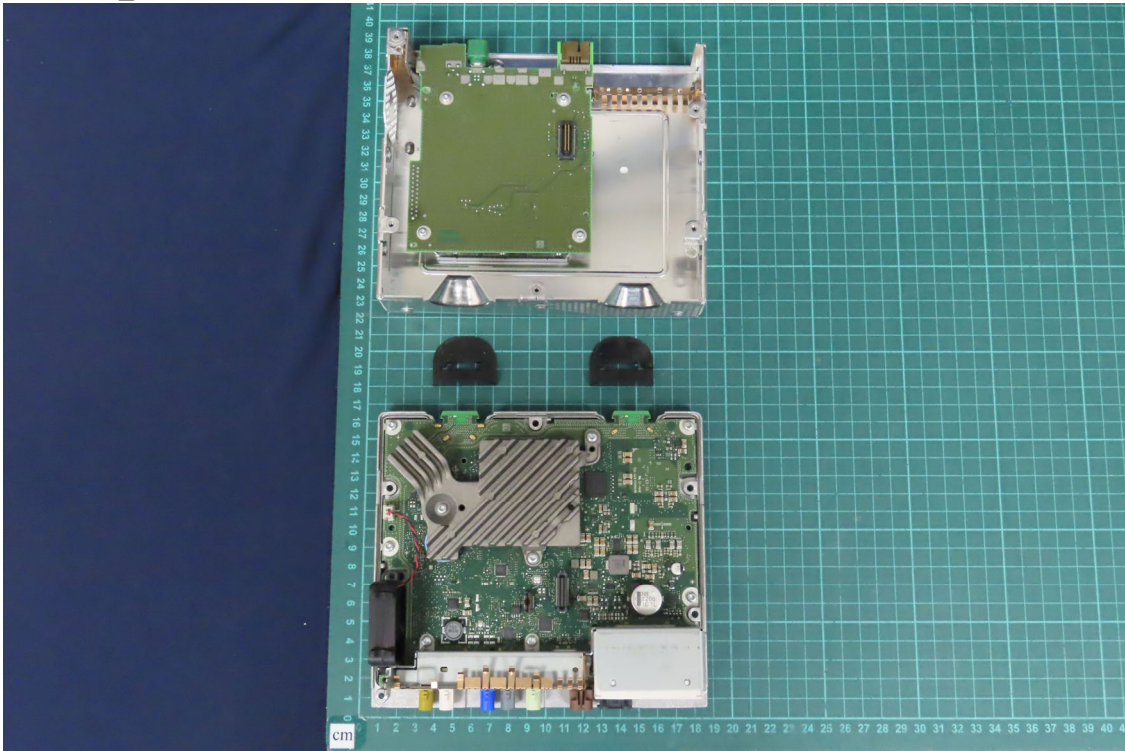
(7) EUT Photo_NA2
