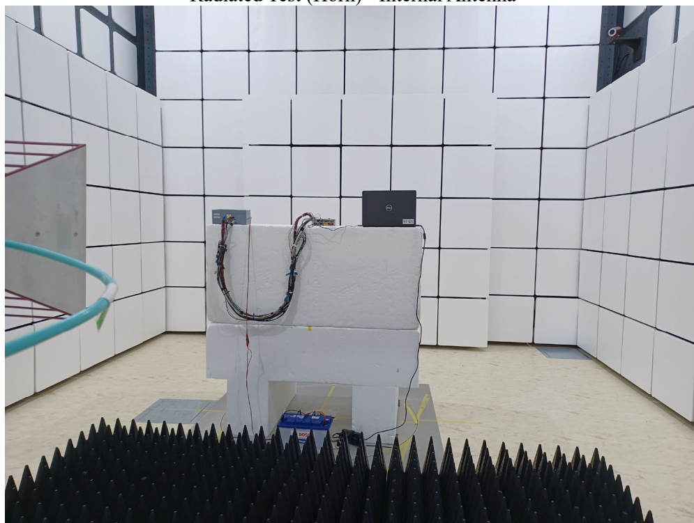
Radiated Test (Horn) - Internal Antenna
