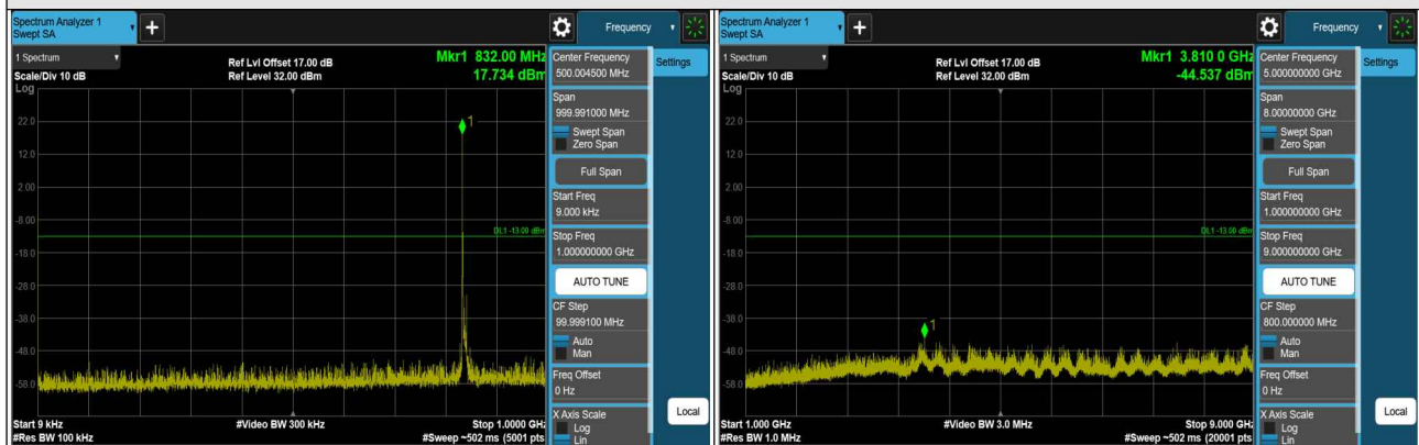
CH 26915 (836.5MHz)
