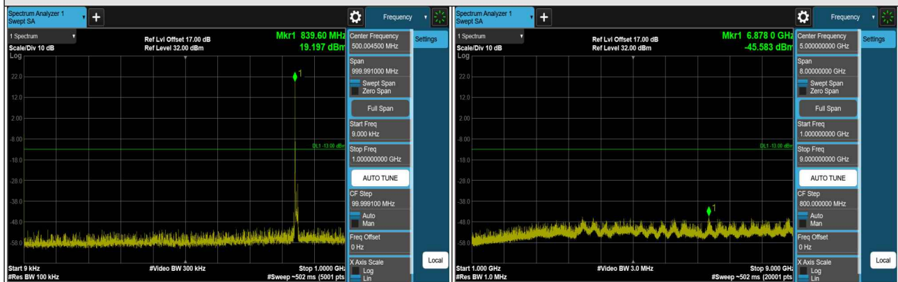
CH 26990 (844MHz)
