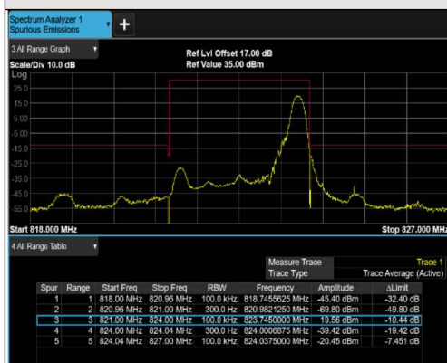
1RB#MAX (822.5MHz)
