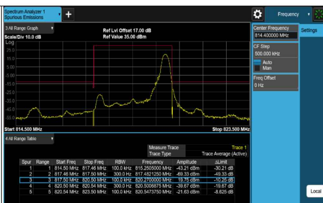
1RB#MAX (819MHz)
