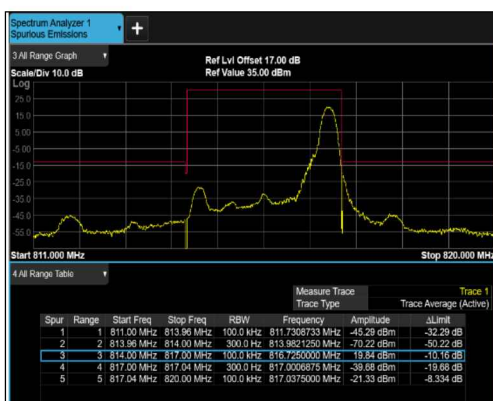
1RB#MAX (815.5MHz)
