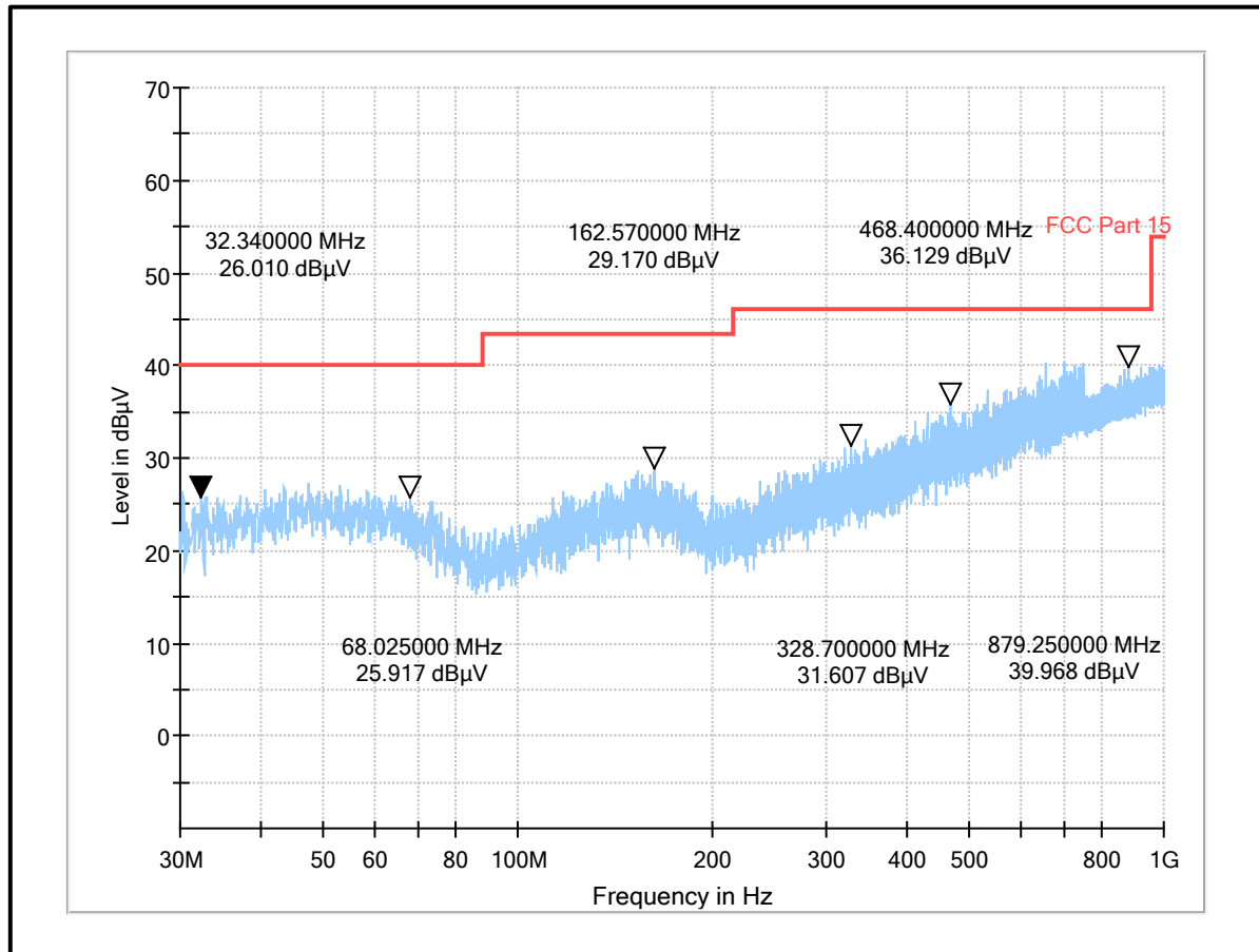
Plot: 30 MHz – 1 GHz: BT-LE / 2 Mbps / PRBS9 / PWR MAX / Top Channel
