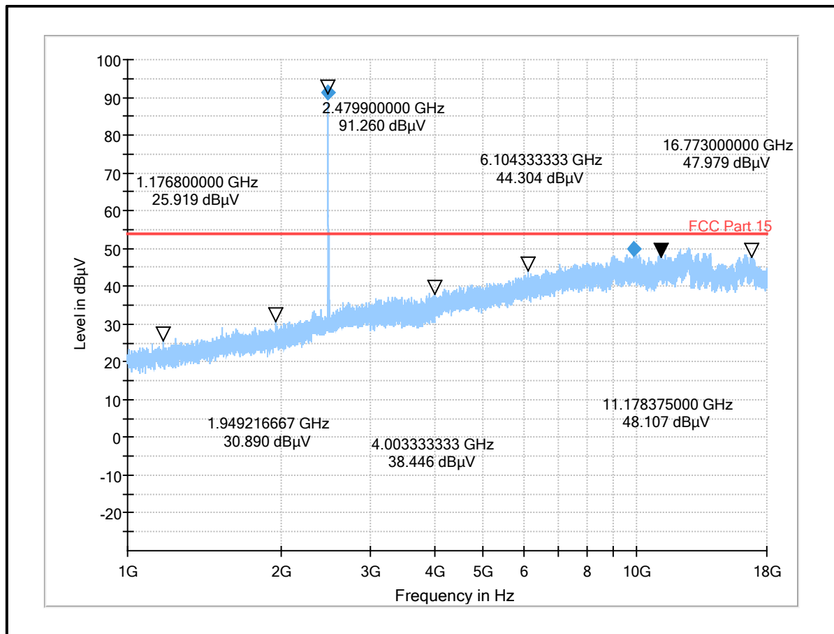
Plot: 1 GHz – 18 GHz: BT-LE / 2 Mbps / PRBS9 / PWR MAX / Top Channel
