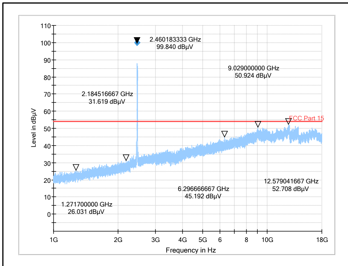
Plot: 1 GHz – 18 GHz: 802.11g / 20 MHz / 54Mbps / Top Channel / PWR 8
