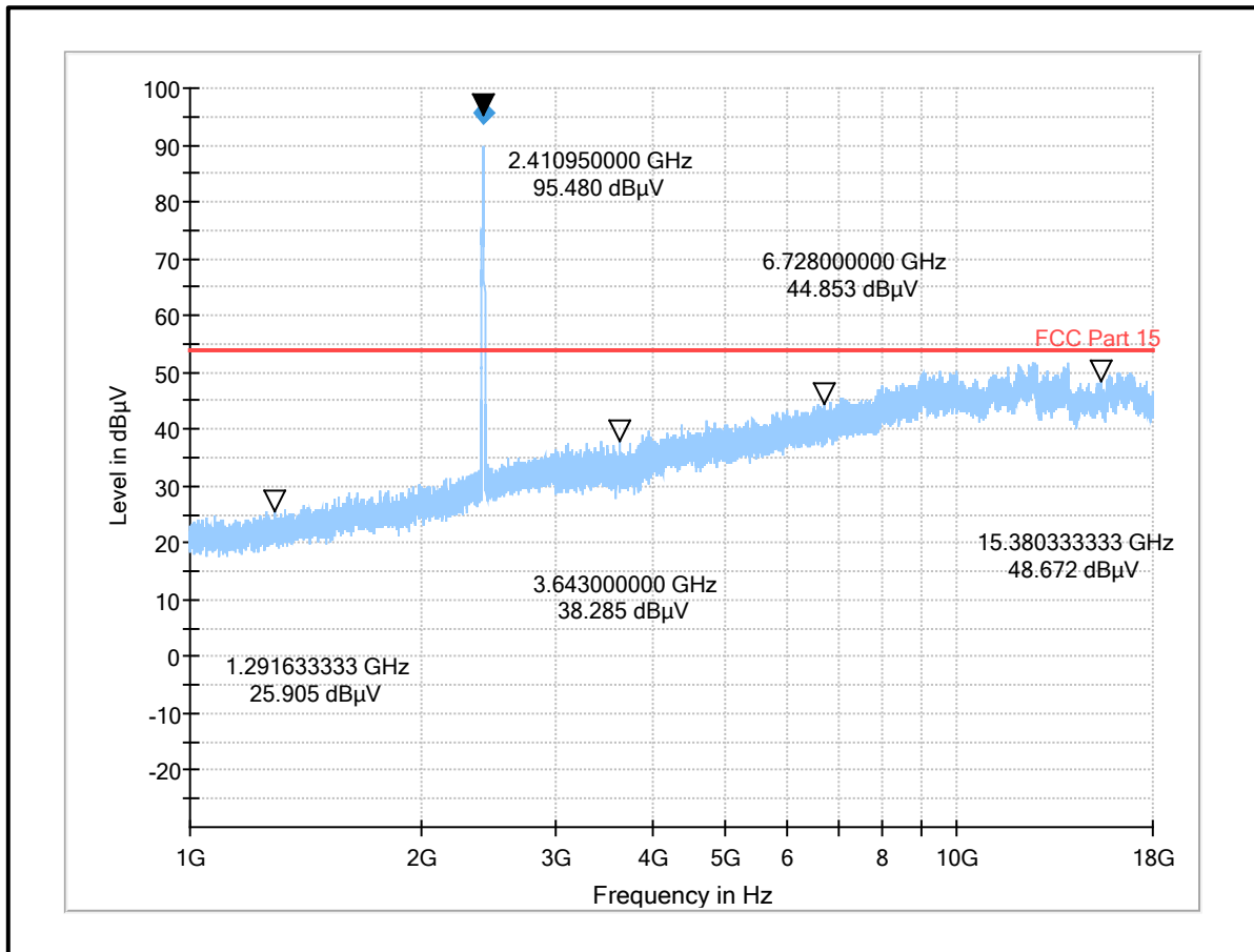
Plot: 1 GHz – 18 GHz: 802.11b / 20 MHz / 1 Mbps / Bottom Channel / PWR 12
