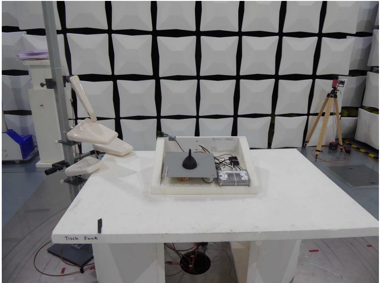
EUT Setup (Emissions < 1 GHz)
