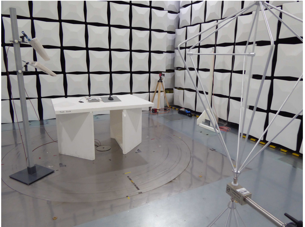
Test setup semi anechoic chamber (30 MHz - 200 MHz)
