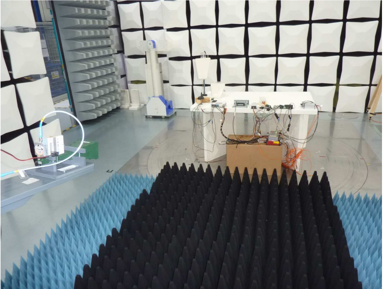
Setup 12 GHz - 18 GHz
