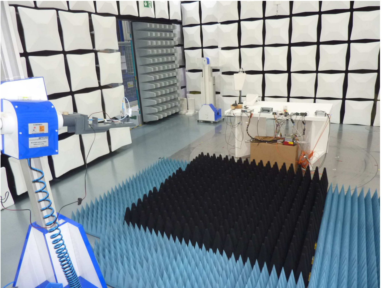
Setup 26.5 GHz – 40 GHz
