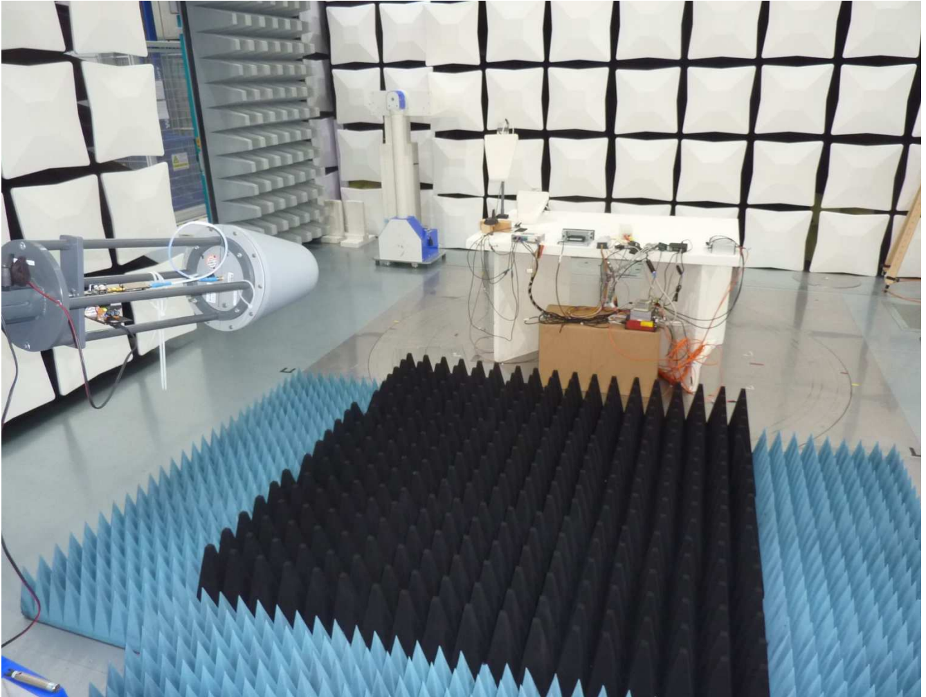
Setup 1 GHz - 12 GHz
