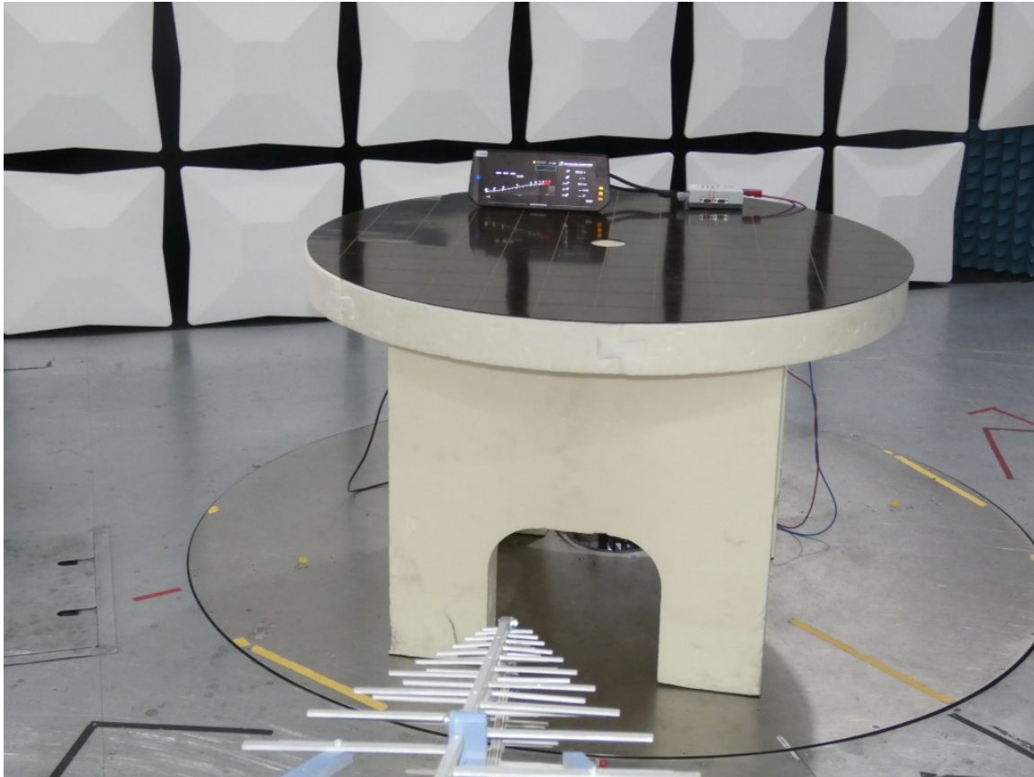
Photo 5: Setup for radiated emissions 30 MHz – 1 GHz, front side view
