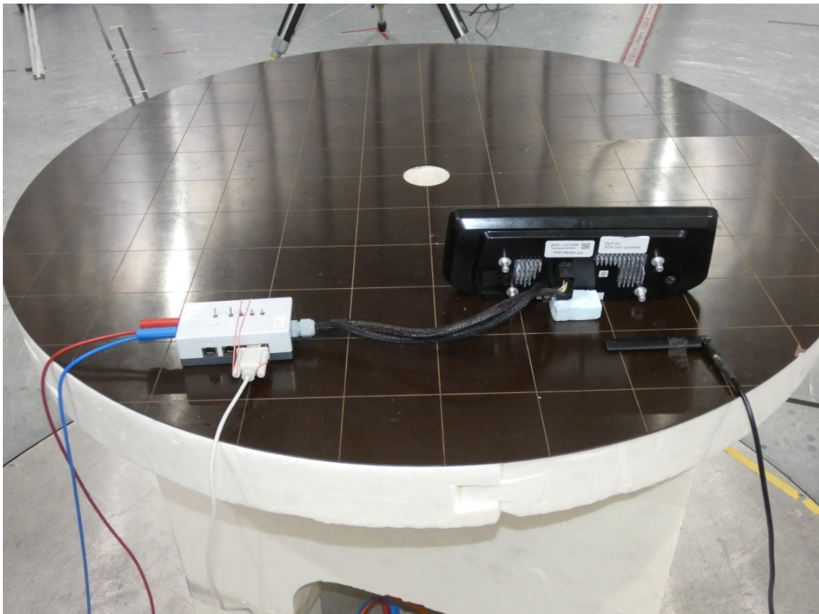
Photo 2: EUT, rear side view
