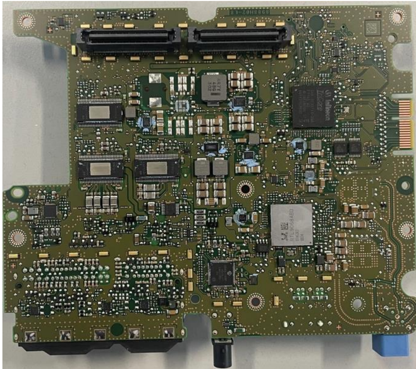
Figure 1. MBCI2LS3PN1 - Base Board – Bottom
