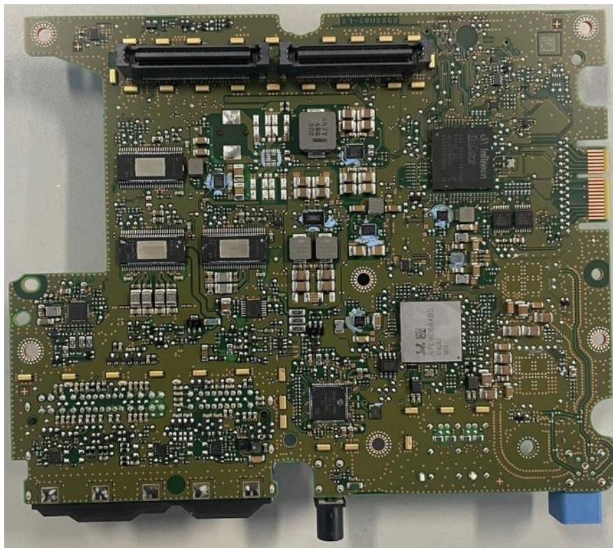
Figure 2. MBCI2LS3PR1 - Base Board – Bottom
