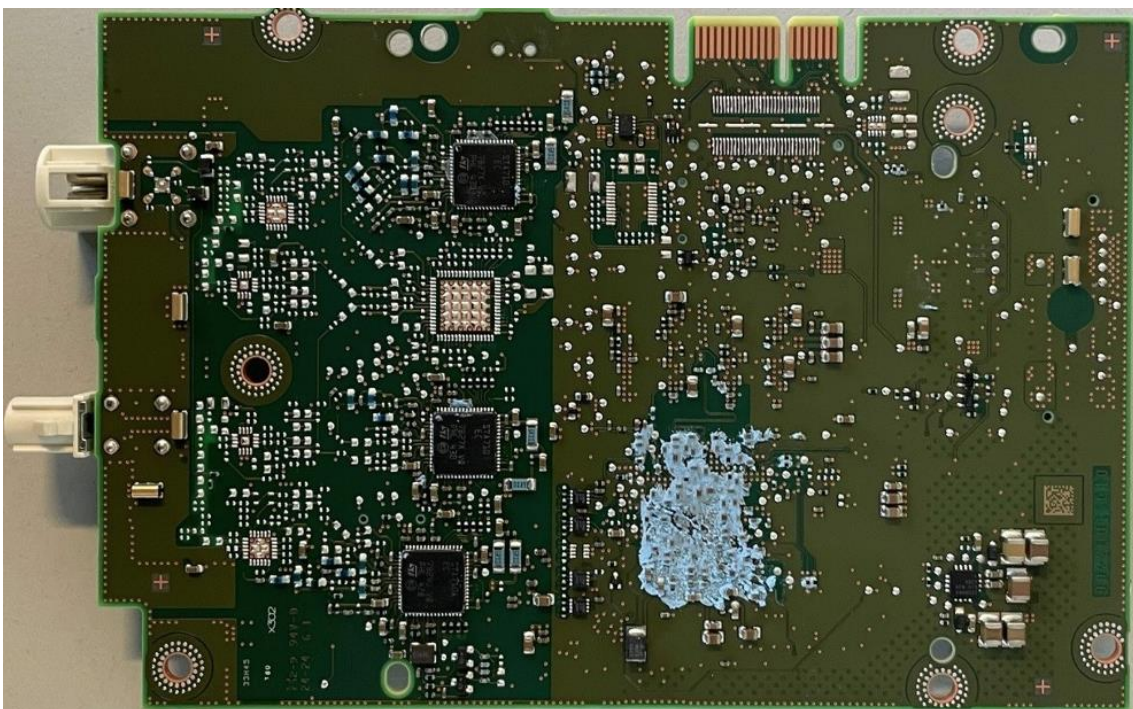
Figure 10. MBCI2LS3PR1 - Country Specific Board – Bottom
