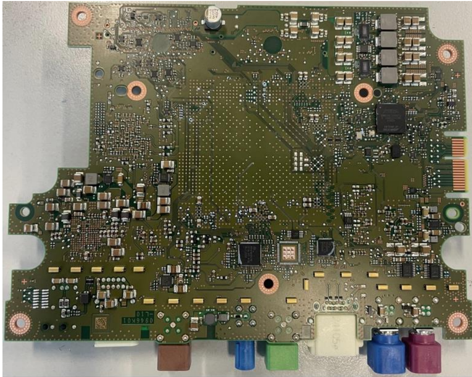
Figure 5. MBCI2LS3PN1 - Multimedia Board – Bottom
