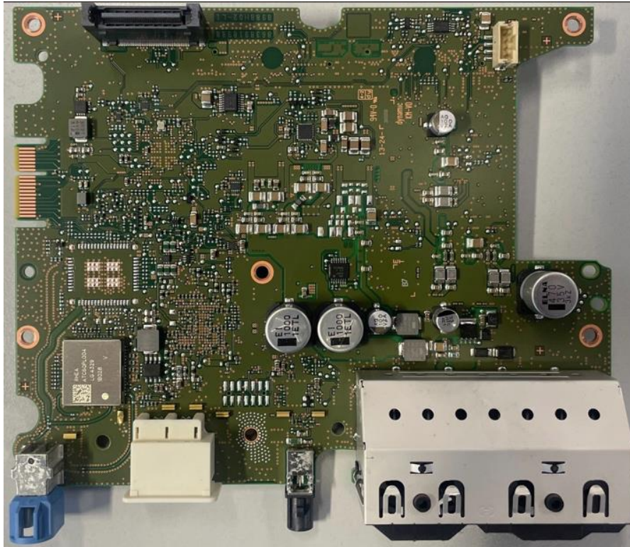
Figure 3. MBCI2LS3PN1 - Base Board – Top
