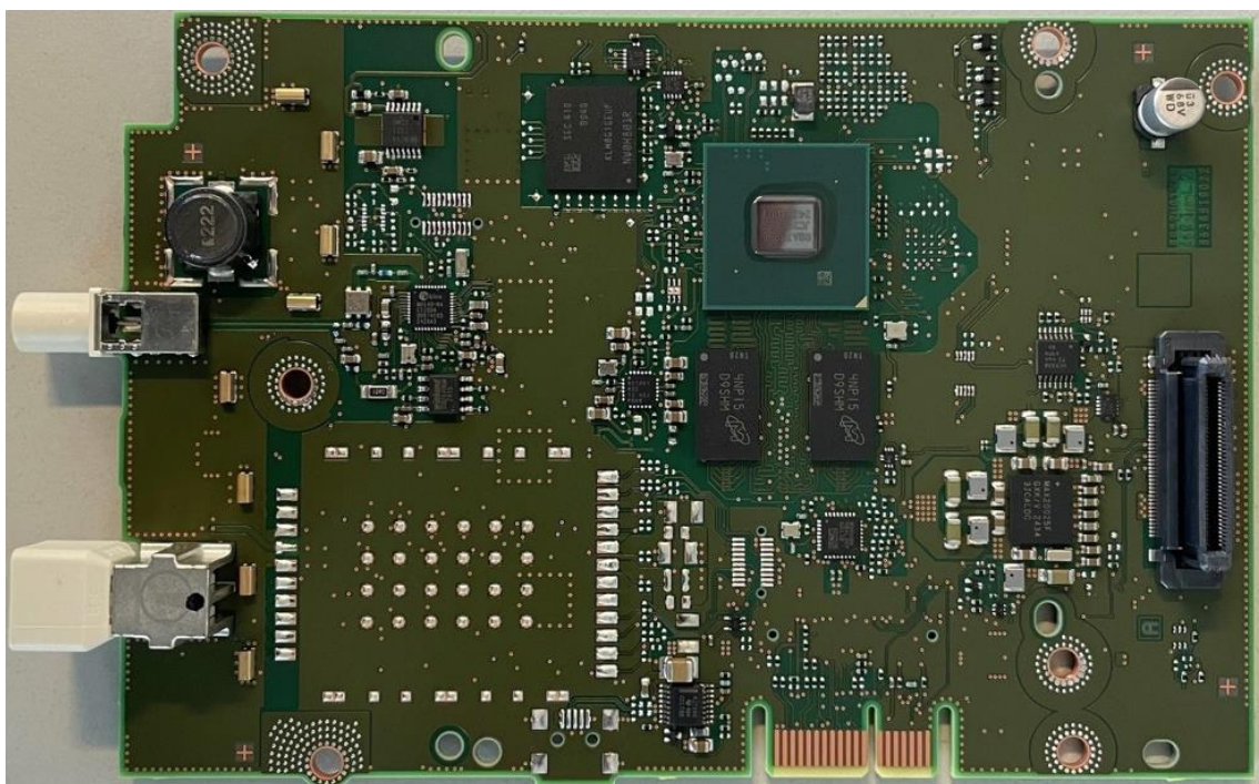
Figure 12. MBCI2LS3PR1 - Country Specific Board – Top
