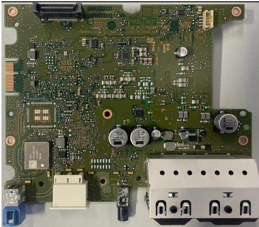
Figure 4. MBCI2LS3PR1 - Base Board – Top
