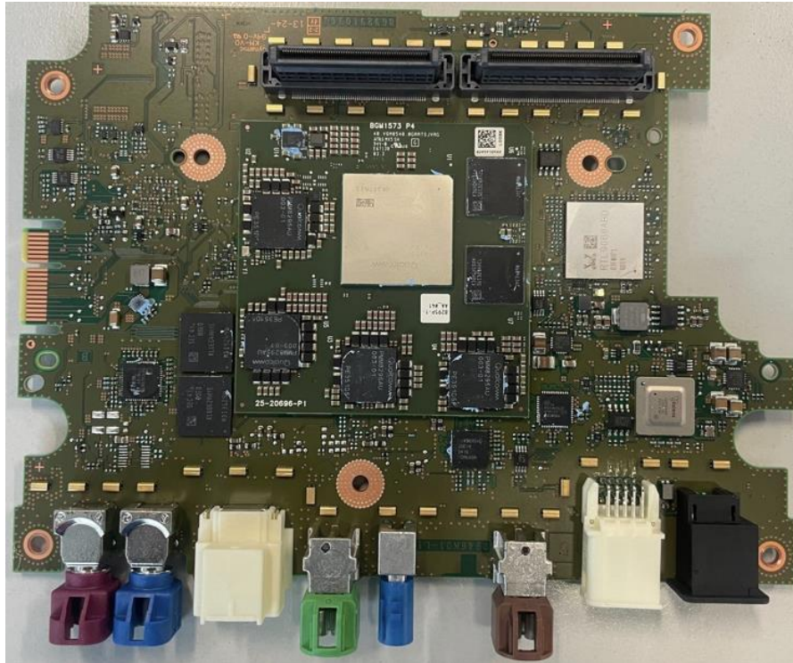
Figure 7. MBCI2LS3PN1 - Multimedia Board – Top
