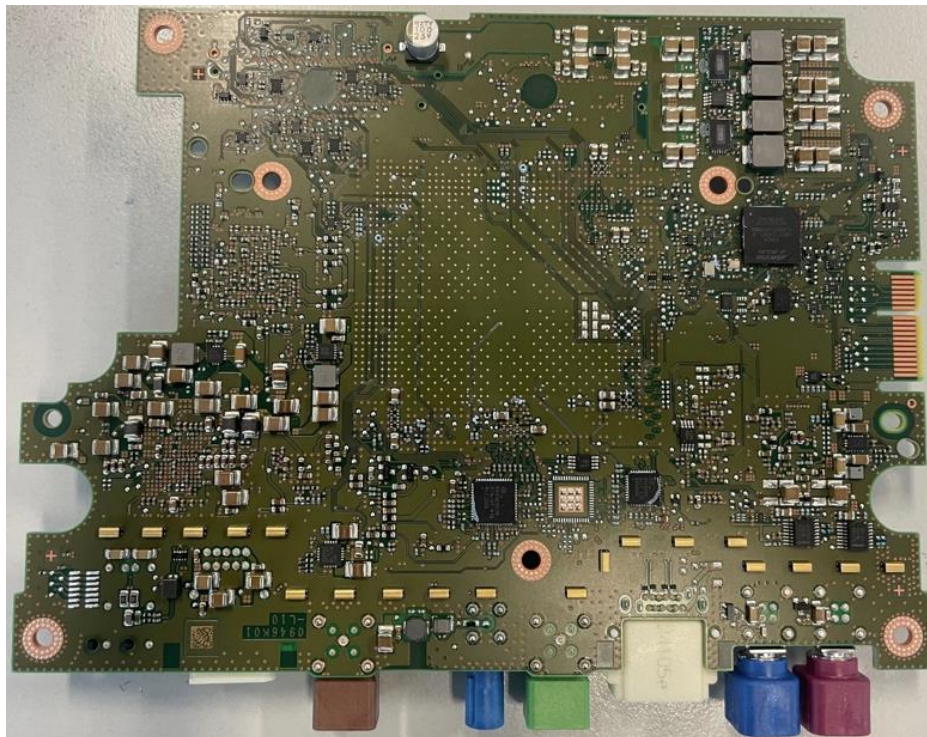
Figure 6. MBCI2LS3PR1 - Multimedia Board – Bottom
