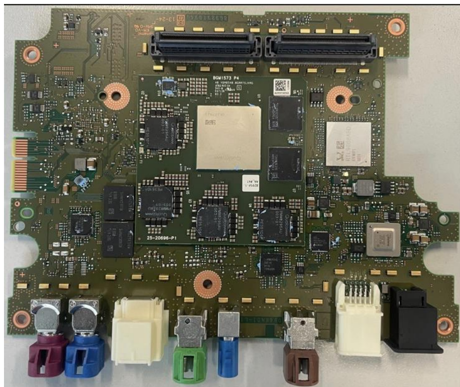
Figure 8. MBCI2LS3PR1 - Multimedia Board – Top
