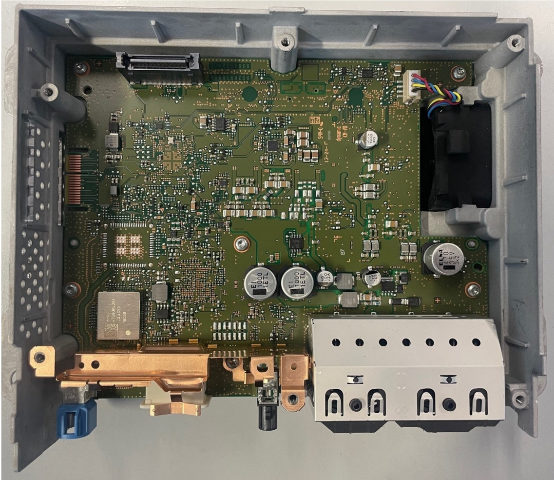
BB Board
