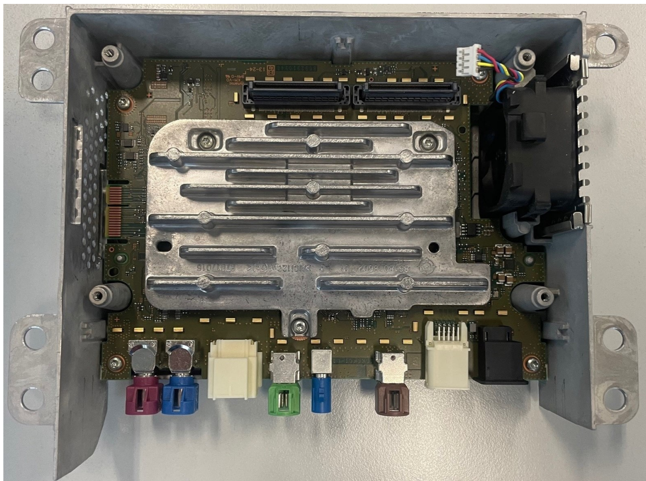
MMB Board
