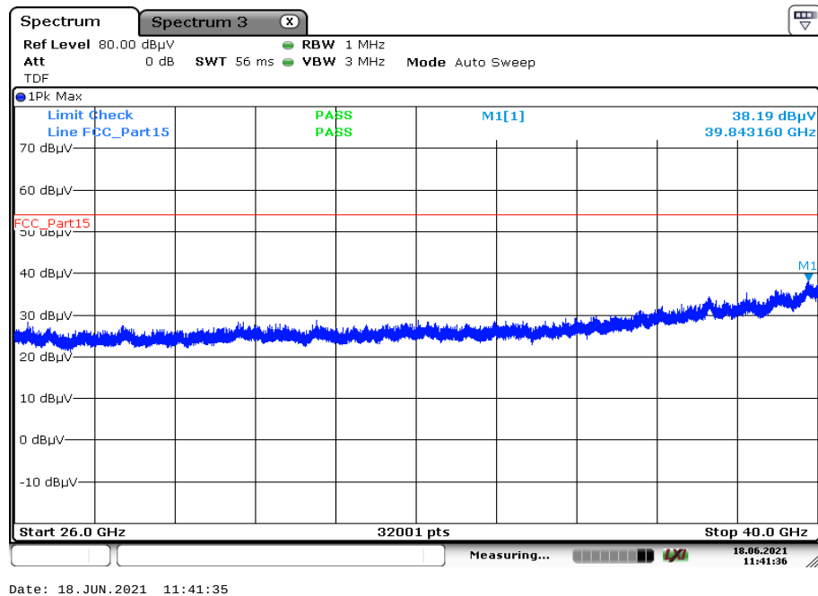
Plot 3: 26 GHz to 40 GHz; vertical & horizontal polarization; U-NII-3; middle channel
