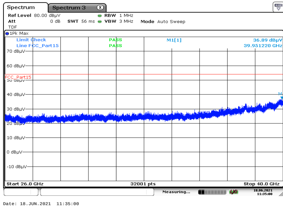
Plot 3: 26 GHz to 40 GHz; vertical & horizontal polarization; U-NII-3; lowest channel
