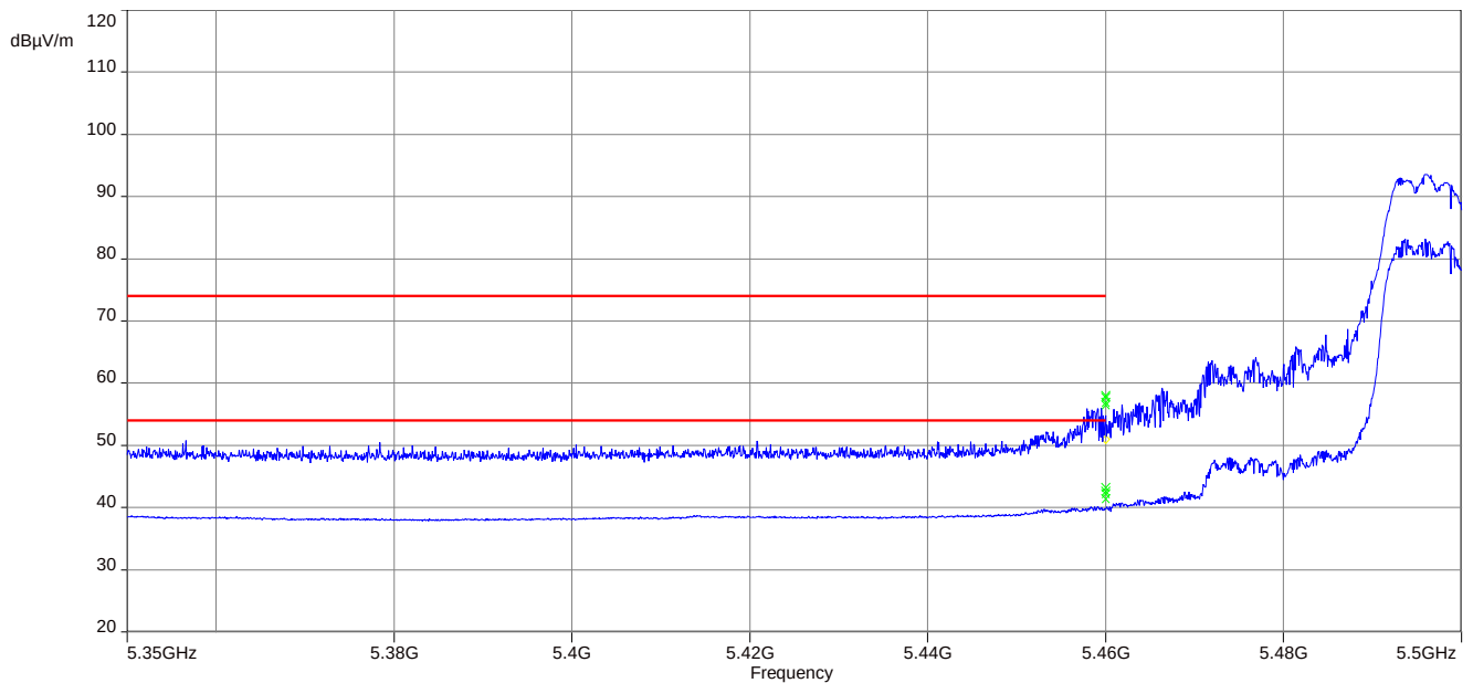
Plot 4: lower band edge; U-NII-2C; lowest channel; 40 MHz channel bandwidth
