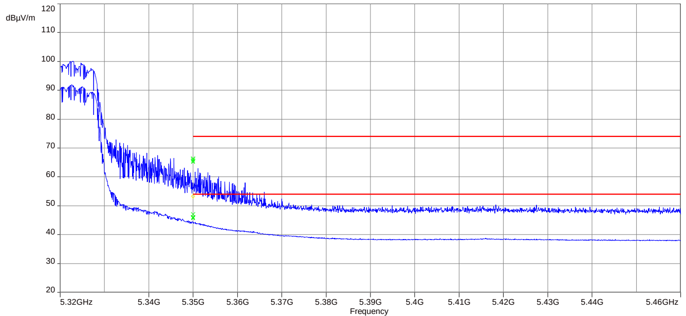
Plot 1: upper band edge; U-NII-2A; highest channel; 20 MHz channel bandwidth
