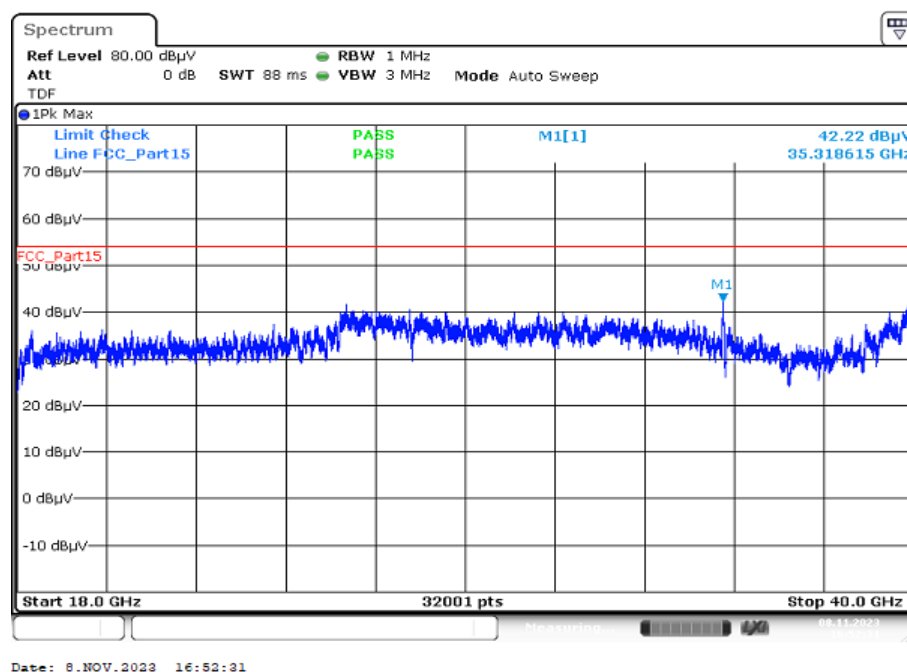
Plot 4: 18 GHz to 40 GHz; vertical & horizontal polarization; valid for all bands, modes and channels
