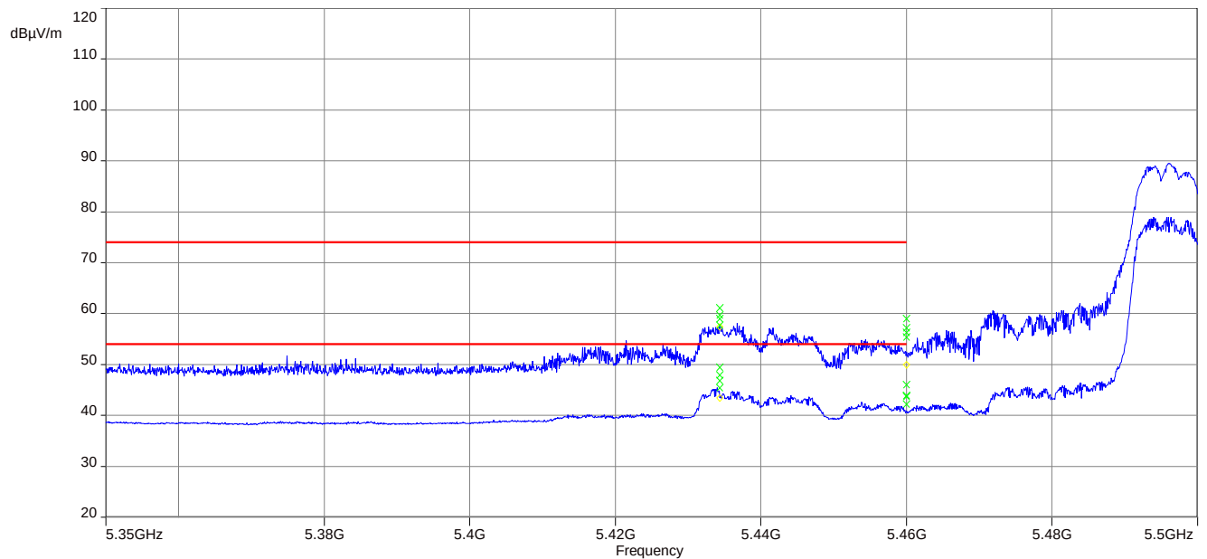
Plot 6: lower band edge; U-NII-2C; lowest channel; 80 MHz channel bandwidth
