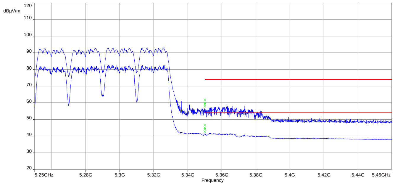
Plot 5: upper band edge; U-NII-2A; middle channel; 80 MHz channel bandwidth
