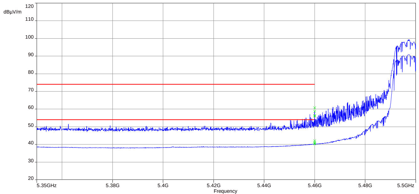
Plot 2: lower band edge; U-NII-2C; lowest channel; 20 MHz channel bandwidth
