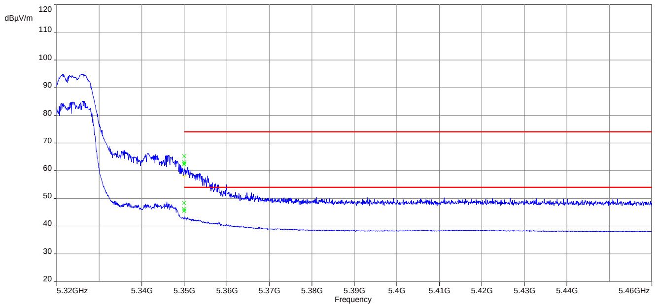
Plot 3: upper band edge; U-NII-2A; highest channel; 40 MHz channel bandwidth
