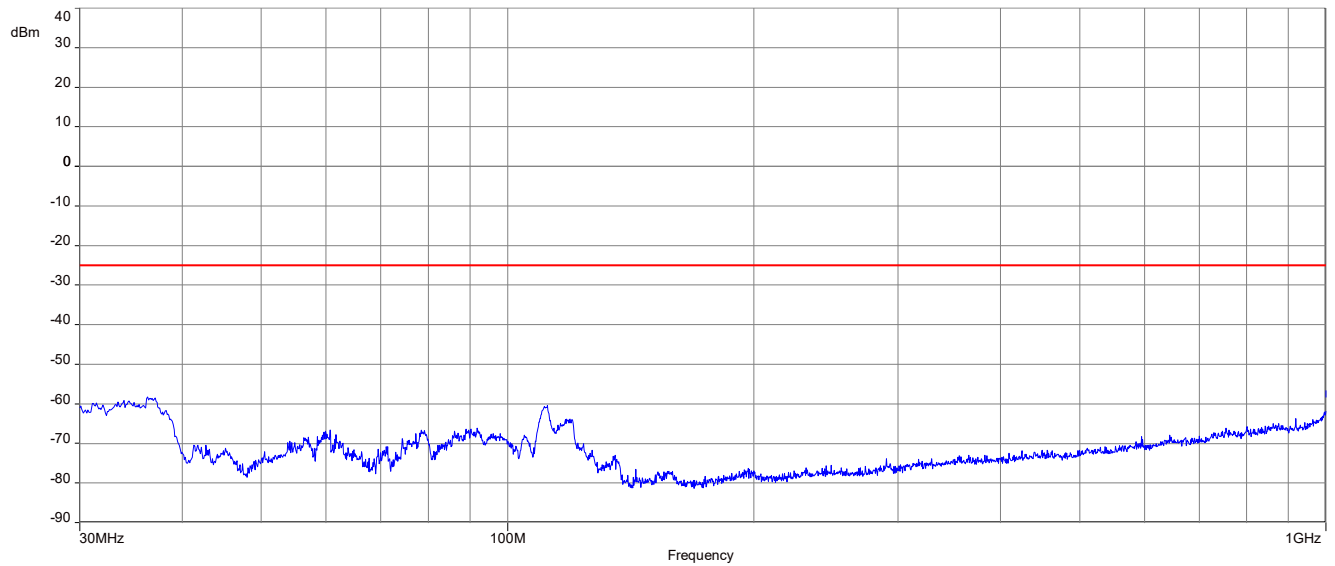
Plot 2: Middle channel (30 MHz – 1 GHz)
