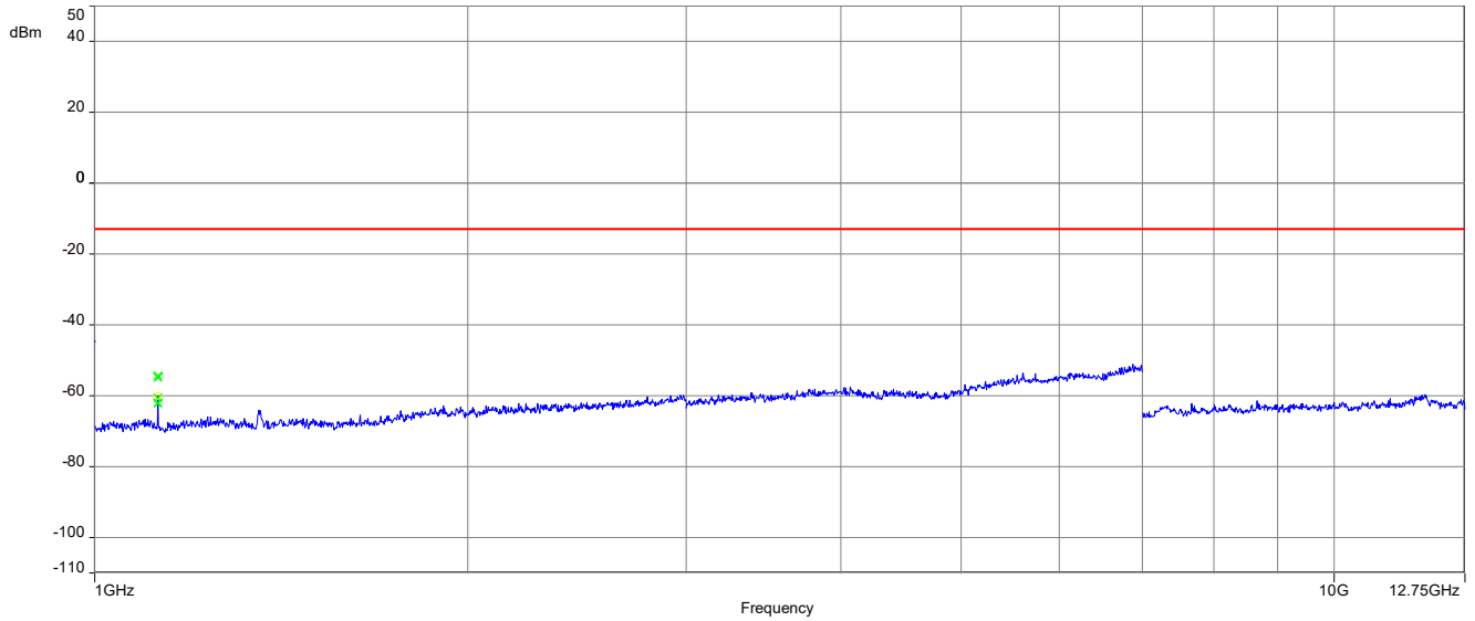
Plot 3: Middle channel (1 GHz to 12.75GHz)
