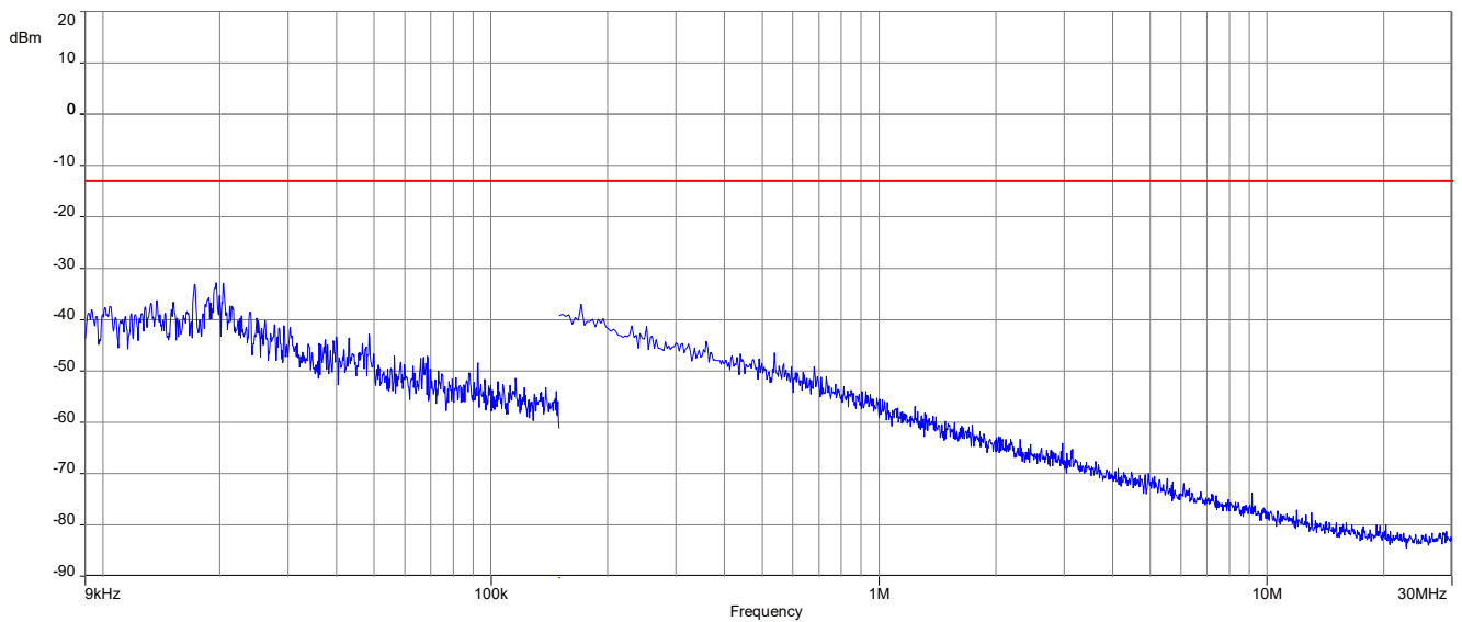
Plot 1: Middle channel (9 kHz - 30 MHz)
