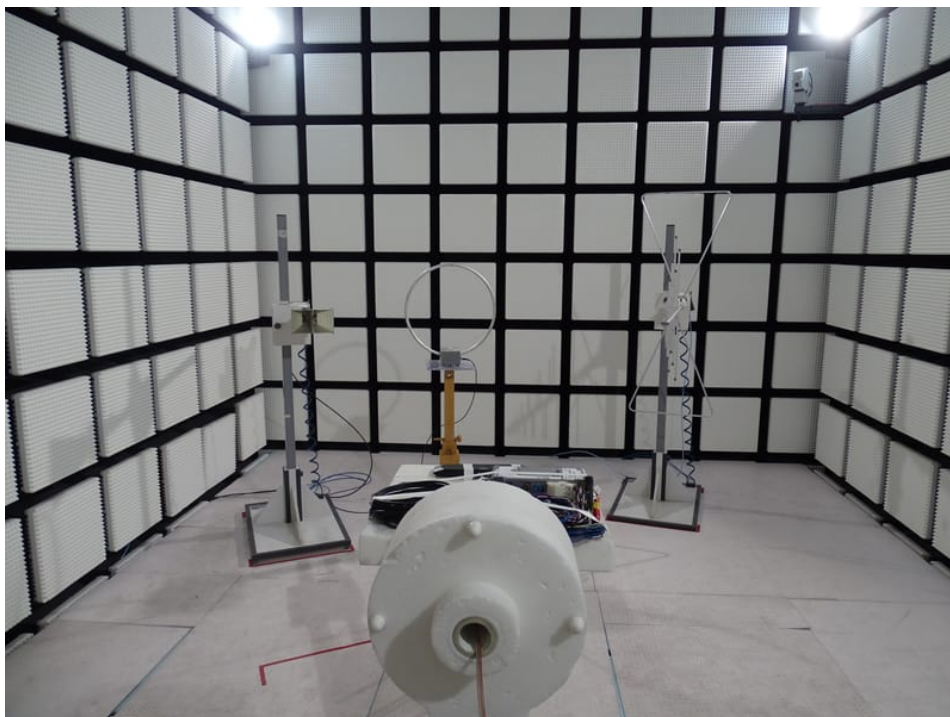
Photo 33: RSE tests with candybar antenna
