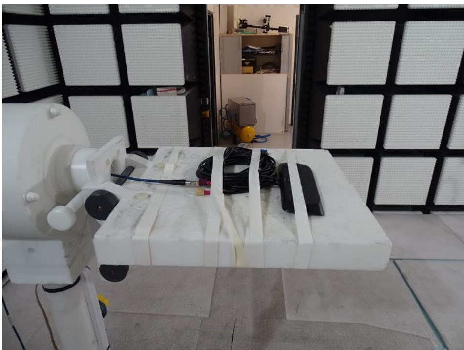
Photo 40: Gain tests with candybar antenna
