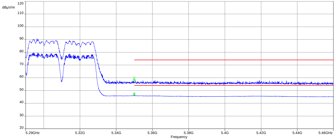
Plot 5: upper band edge; U-NII-2A; middle channel; 80 MHz channel bandwidth
