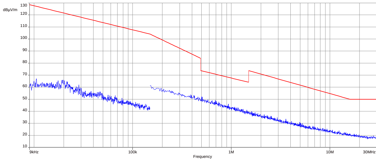
Plot 3: 9 kHz to 30 MHz, U-NII-2C; highest channel
