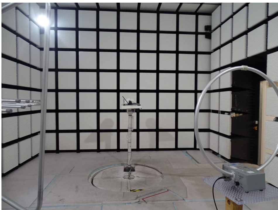
Photo 6: RSE tests with Supercombo antenna
