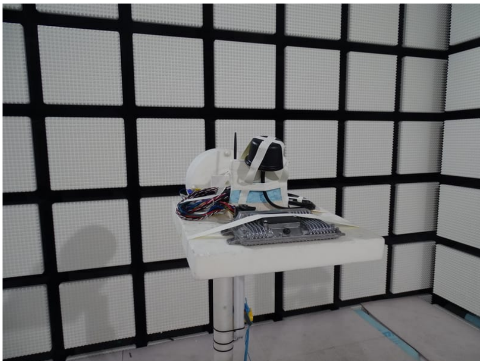
Photo 14: RSE tests with Puck antenna
