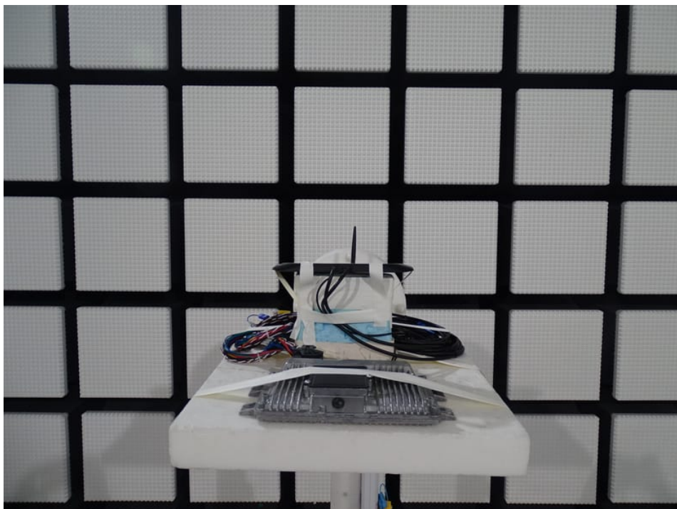
Photo 26: RSE tests with candybar antenna
