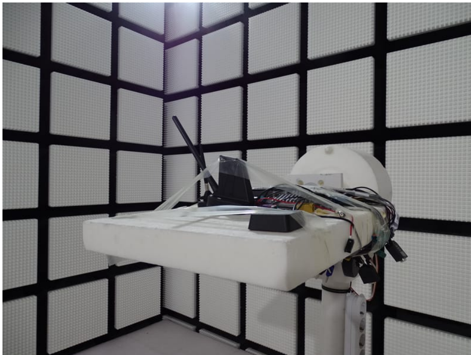
Photo 3: RSE tests with Supercombo antenna
