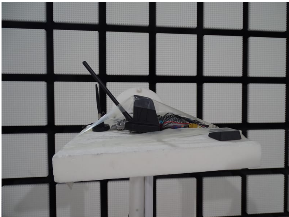
Photo 2: RSE tests with Supercombo antenna
