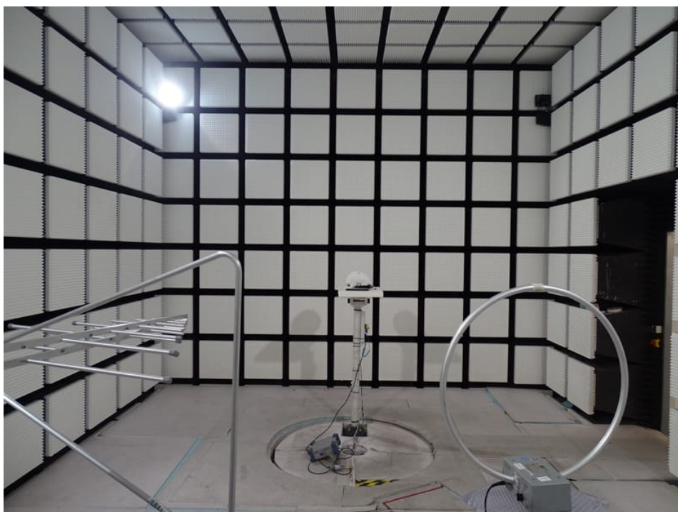
Photo 28: Gain tests with candybar antenna
