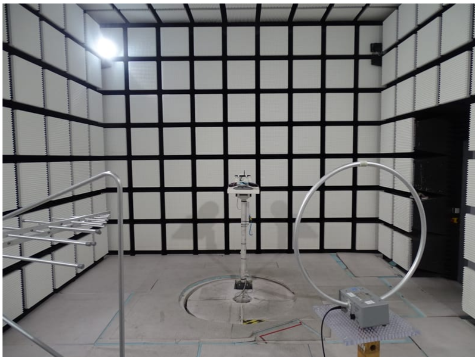
Photo 27: RSE tests with candybar antenna
