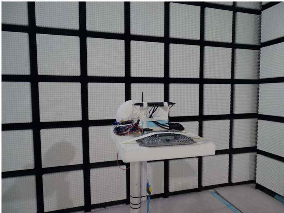
Photo 25: RSE tests with candybar antenna
