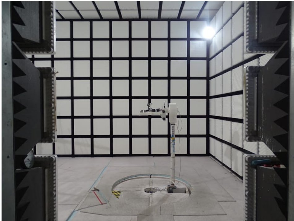
Photo 23: RSE tests with candybar antenna
