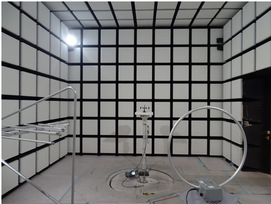
Photo 11: Gain tests with Supercombo antenna
