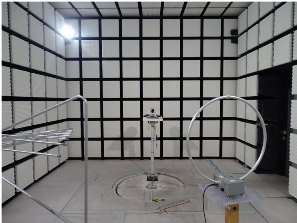
Photo 17: RSE tests with Puck antenna
