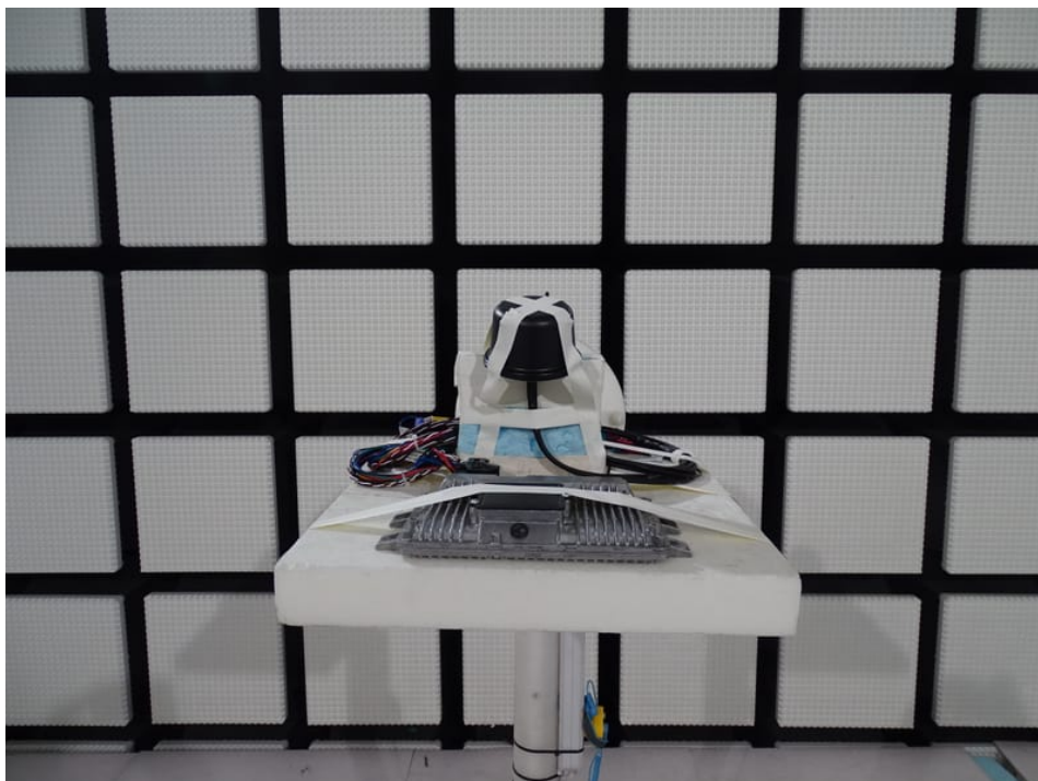
Photo 15: RSE tests with Puck antenna
