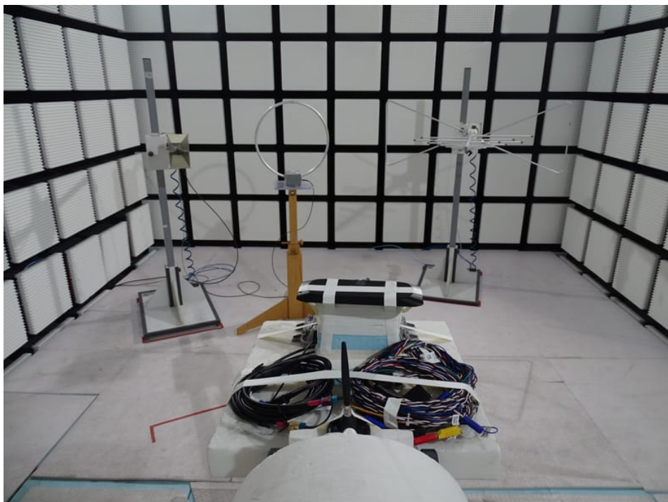
Photo 24: RSE tests with candybar antenna
