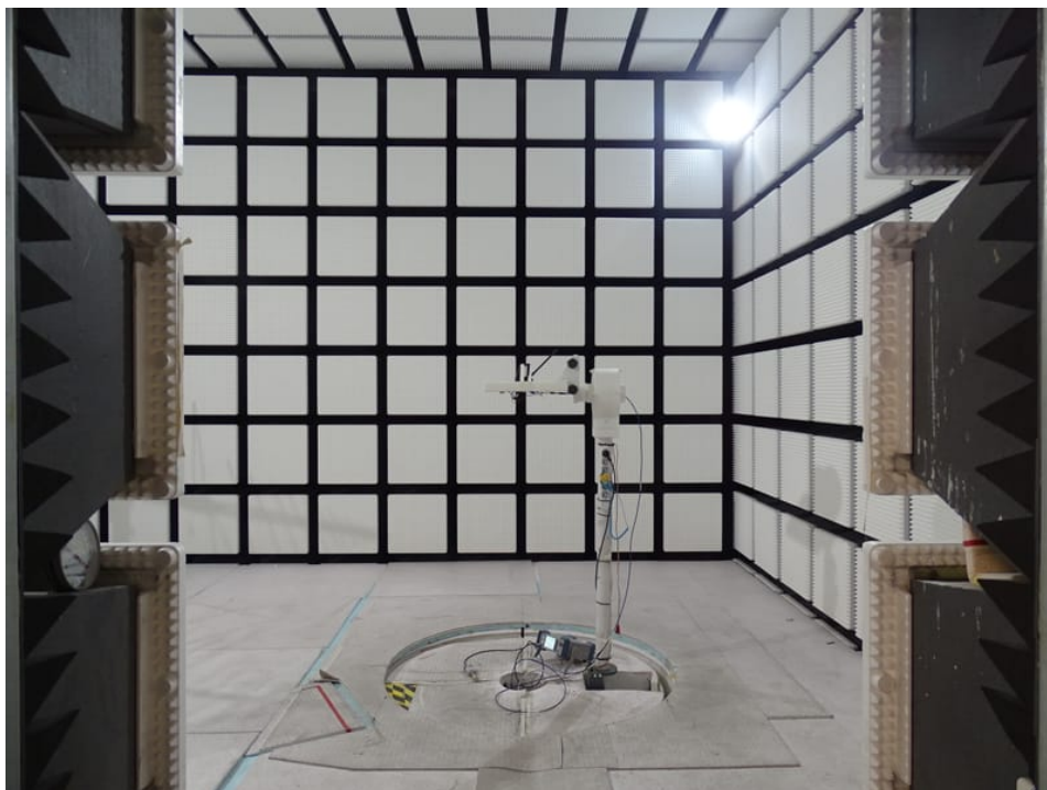
Photo 7: Gain tests with Supercombo antenna
