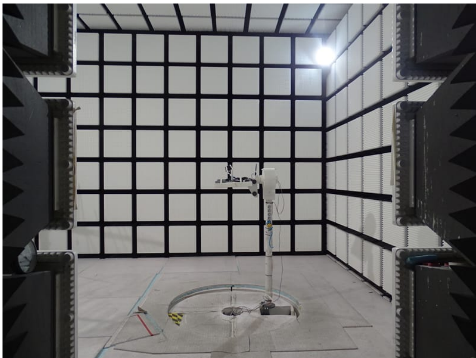
Photo 12: RSE tests with Puck antenna
