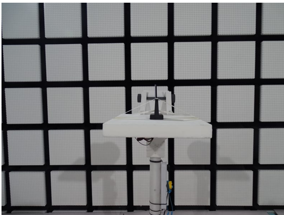
Photo 10: Gain tests with Supercombo antenna
