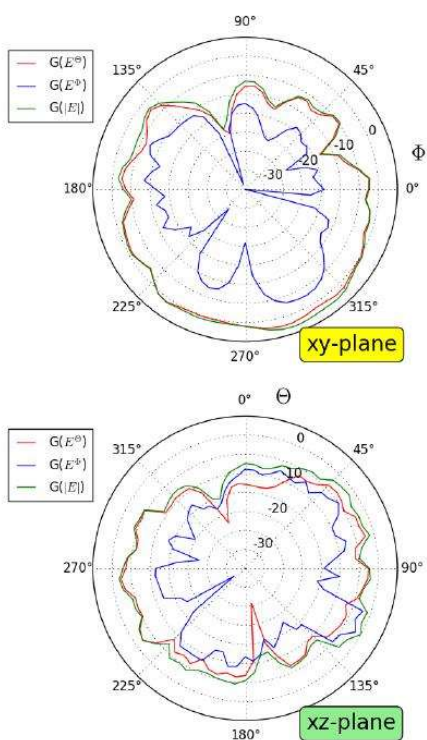
Figure 5 Wlan 5 GHz, 5502,5 MHz
