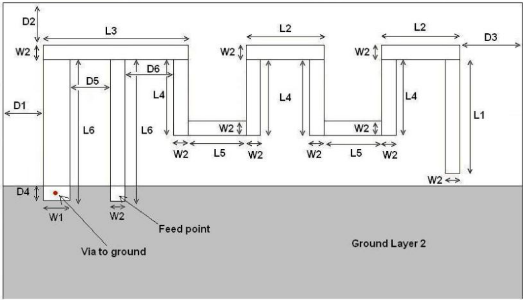
Figure 3: Antenna Dimensions
