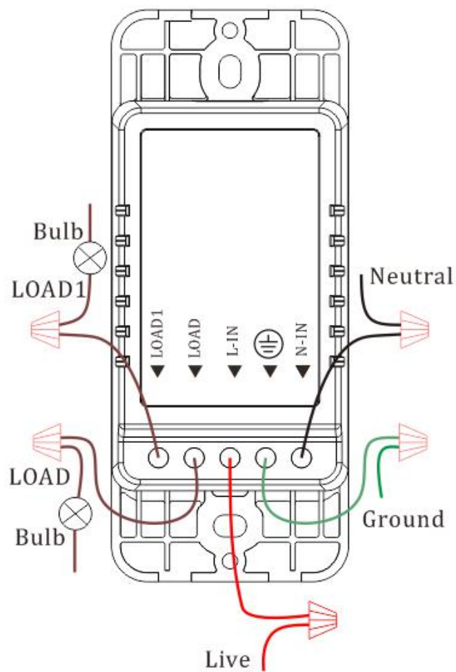
Wiring diagram
