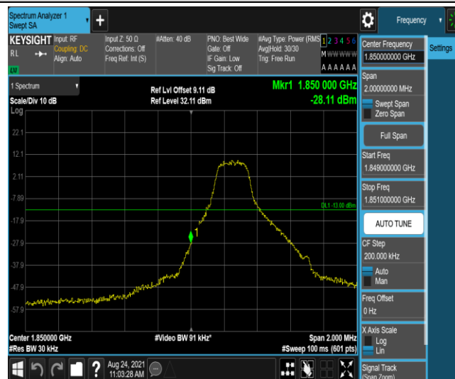
Band2-1.4MHz-QPSK-18607-1RB#5
