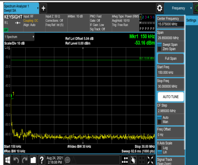
Band4-10MHz-QPSK-20350-1RB#0-Range3:30~1000MHz
