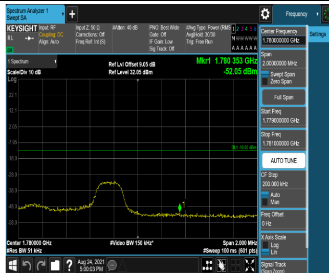
Band66-3MHz-16QAM-132657-1RB#14
