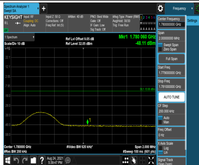
Band66-10MHz-16QAM-132622-1RB#49
