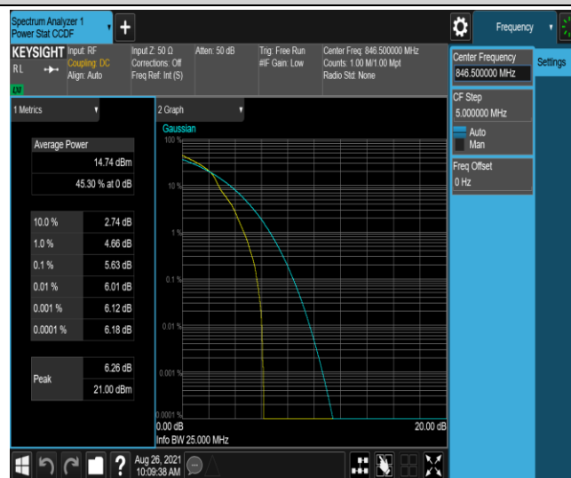
Band5-5MHz-16QAM-20625-25RB#0
