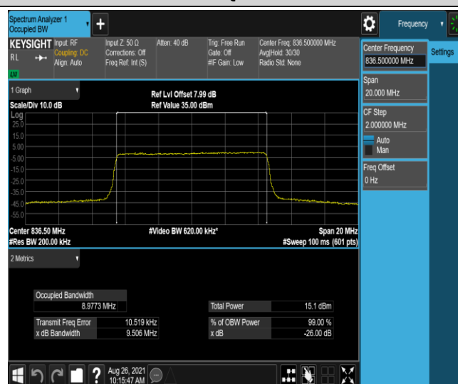
Band5-10MHz-16QAM-20600-50RB#0
