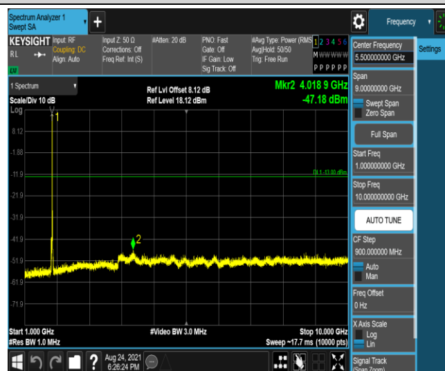
Band66-20MHz-16QAM-132572-1RB#0-Range4:1000~10000MHz
