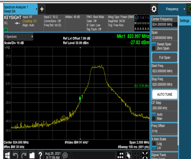
Band5-1.4MHz-16QAM-20407-1RB#5
