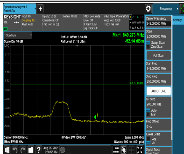
Band5-3MHz-16QAM-20635-1RB#14
