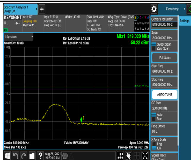
Band5-5MHz-16QAM-20625-1RB#24
