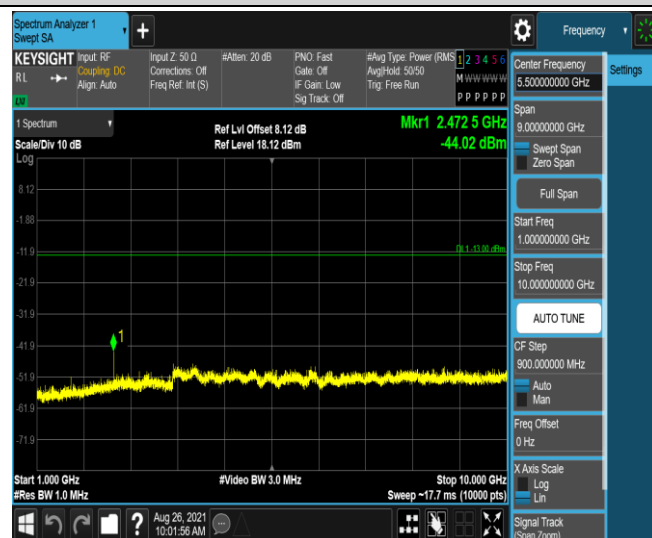
Band5-5MHz-16QAM-20525-1RB#0-Range1:0.009~0.15MHz
