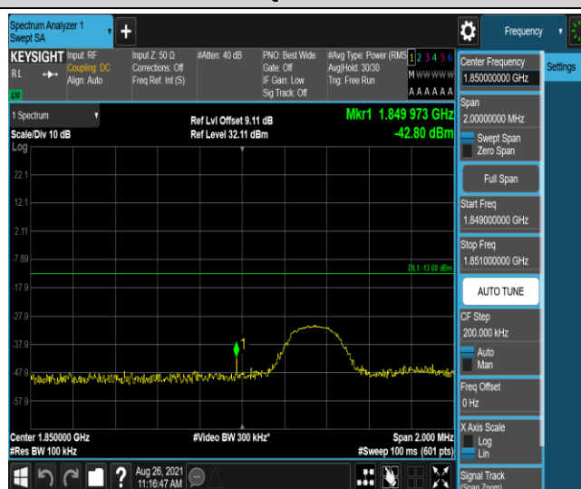
Band25-5MHz-QPSK-26065-25RB#0
