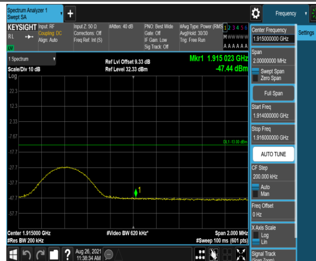
Band25-10MHz-16QAM-26640-1RB#49
