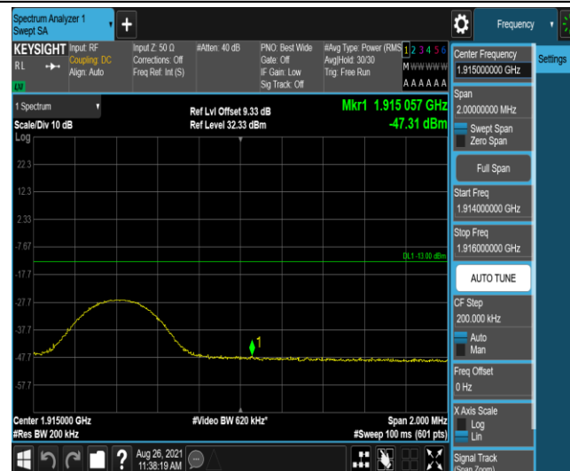
Band25-10MHz-QPSK-26640-1RB#49
