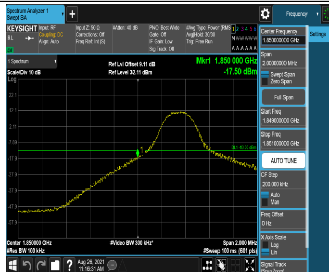
Band25-5MHz-16QAM-26065-1RB#24
