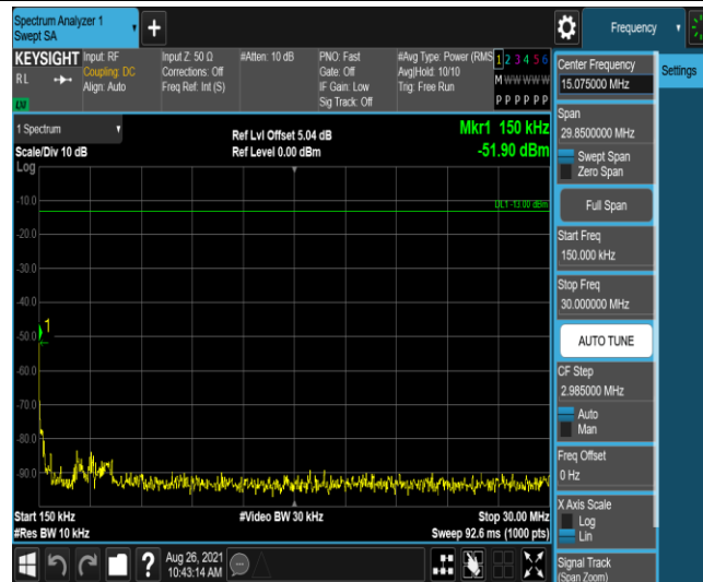
Band25-1.4MHz-QPSK-26683-1RB#0-Range3:30~1000MHz
