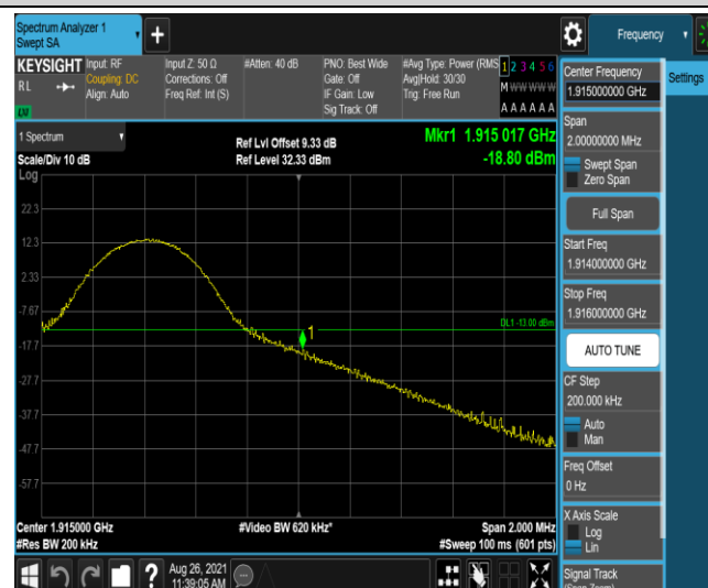
Band25-10MHz-16QAM-26640-50RB#0
