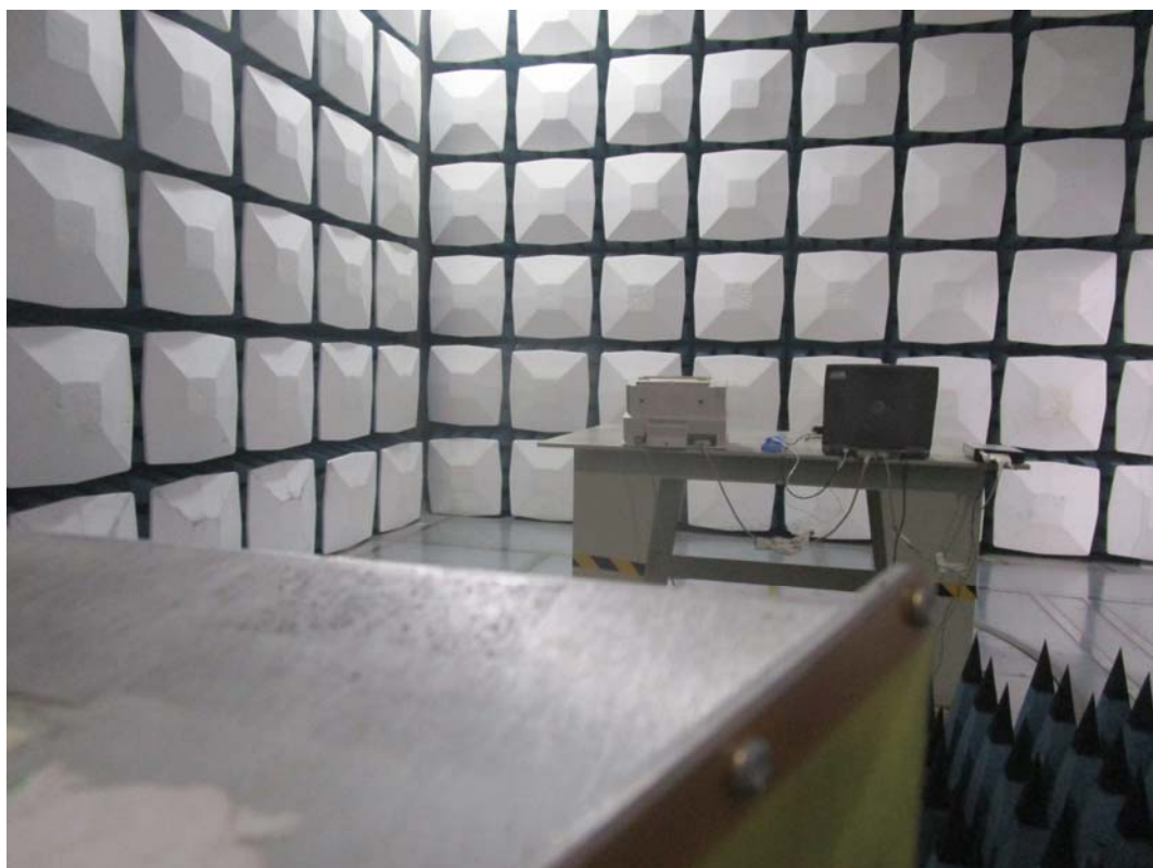
Radiated Emission Above 1GHz Side View
