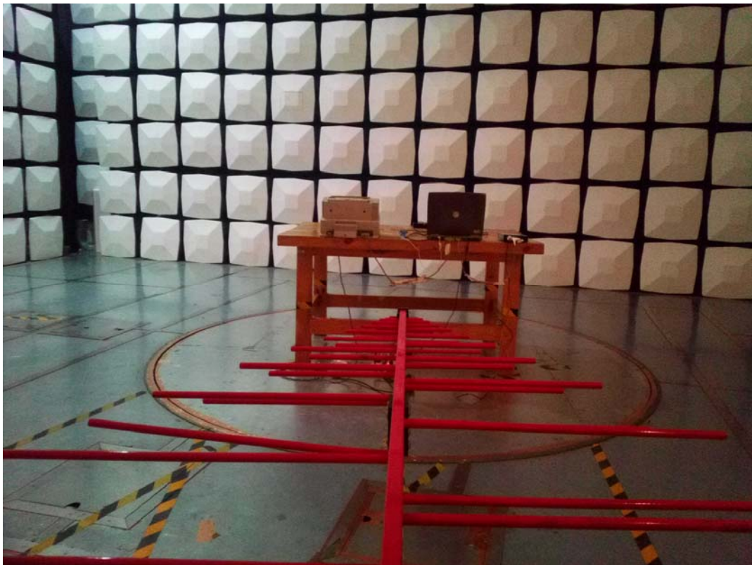
Radiated Emission Below 1GHz Side View
