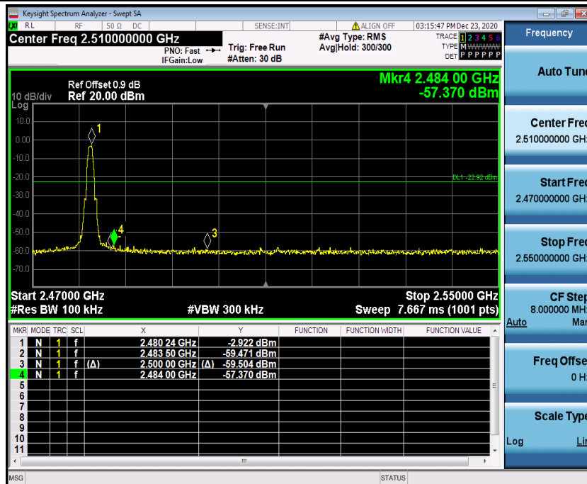
BLE_Ant1_High_2480
