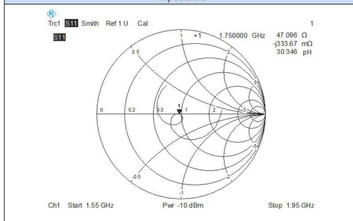
Impedance
