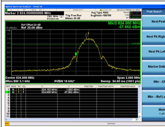
GSM850(EDGE), CH128, 824.2MHz
