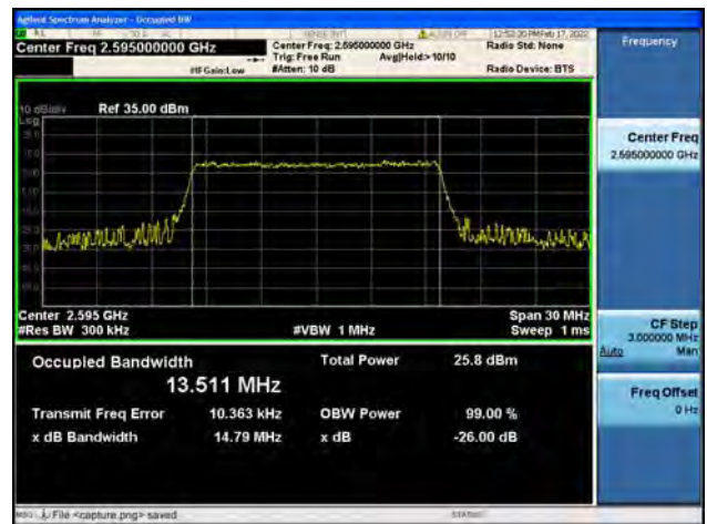
Band38 / 15MHz / Mid CH / 64QAM
