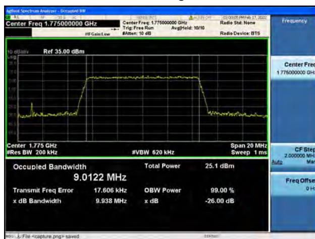
Band66 / 10MHz / High CH / 64QAM
