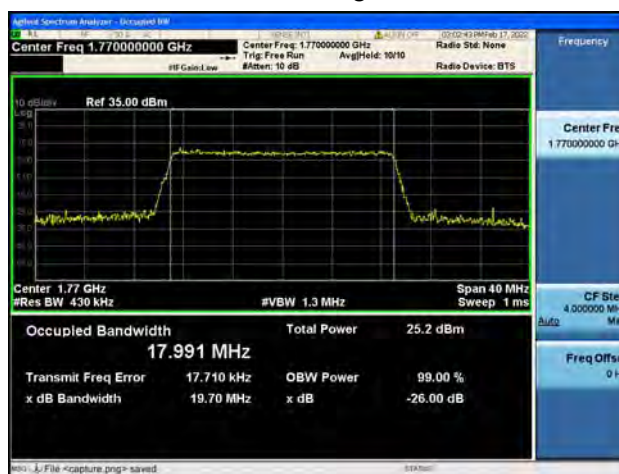
Band66 / 20MHz / High CH / 64QAM
