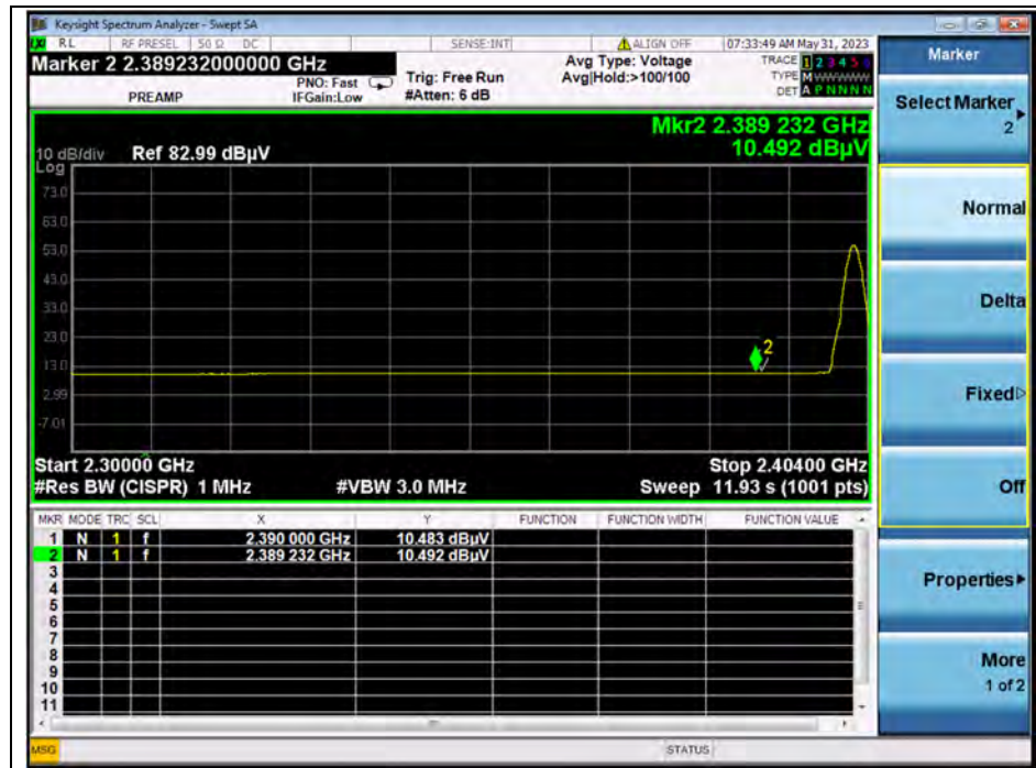
(AVERAGE, Channel 0)
