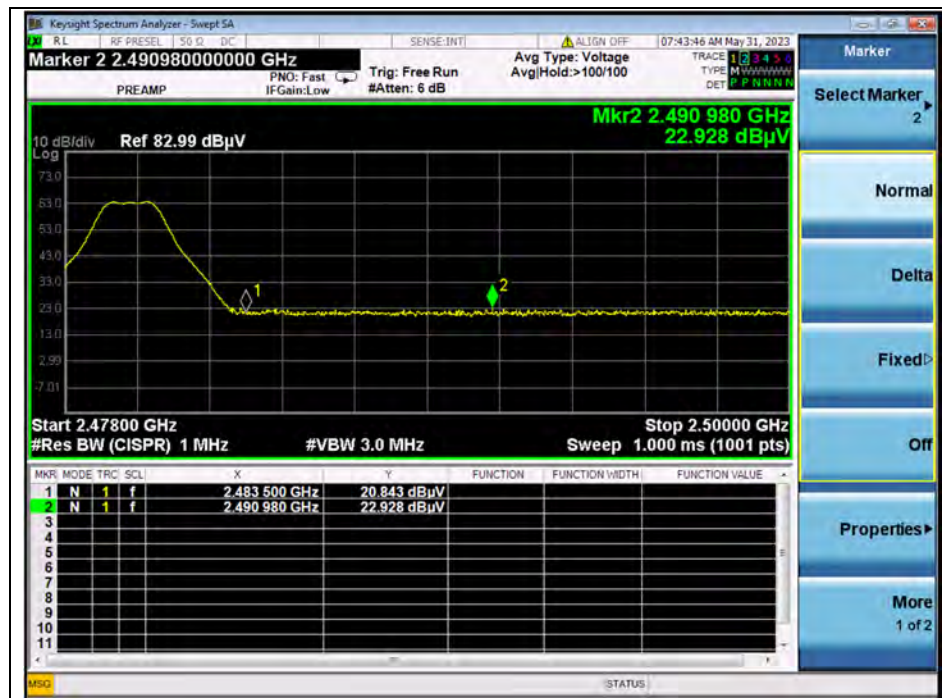
(PEAK, Channel 39)
