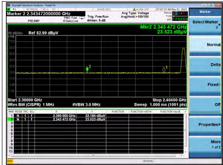
(PEAK, Channel 0)
