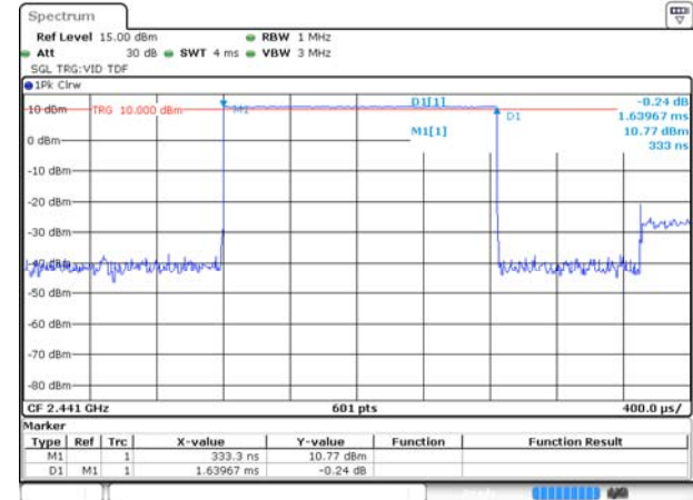
GFSK DH3
