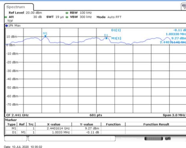
8-DPSK
